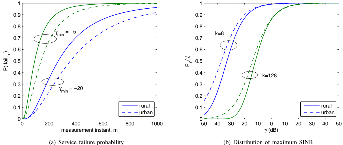
Fig. 9. Urban macrocell versus rural macrocell.
