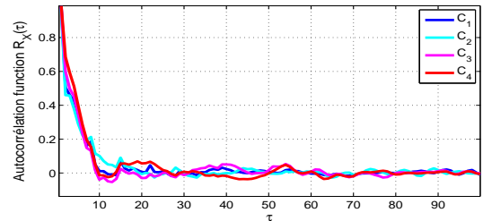
Fig. 6. Autocorrelation function R_X for each class C_p .
