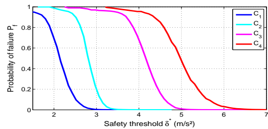
Fig. 10. Evolution of P_f(\delta^*) as function of \delta^* .
