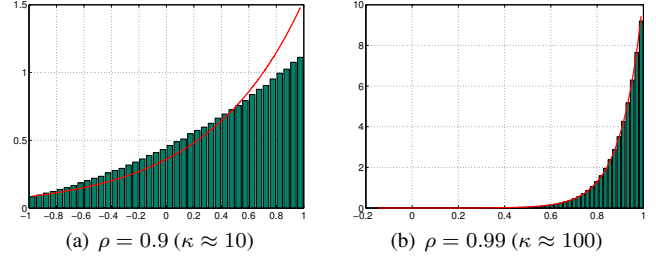
Fig. 1. Green bars: histogram of the tangent part t = \mathbf{x}_n^T \boldsymbol{\mu} ( 10^6 samples); Red line: pdf of the vMF based approximation \tilde{t} = \tilde{\mathbf{x}}_n^T \boldsymbol{\mu} where \tilde{\mathbf{x}}_n \sim M_p(\boldsymbol{\mu}, \tilde{\kappa}_n)
