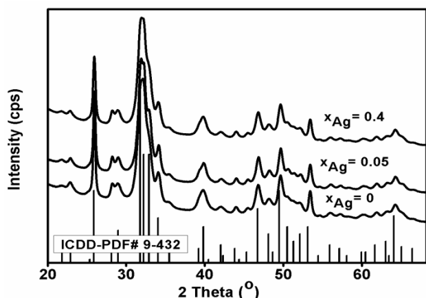
Fig. 1. Comparative representation of the experimental XRD patterns of the Ag:HAp samples synthesized x_{Ag} = 0 , x_{Ag} = 0.05 , and x_{Ag} = 0.4 , and the characteristic lines of hydroxyapatite according to the ICDD - PDF number 9-432
