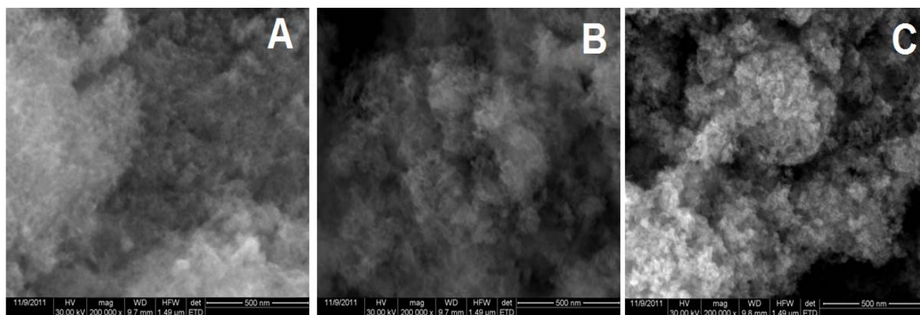
Fig. 2. SEM images of the Ag:HAp samples with x_{Ag} = 0 (A), x_{Ag} = 0.05 (B) and x_{Ag} = 0.4 (C).
