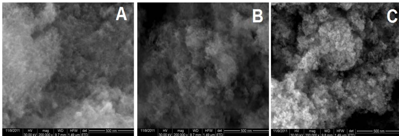
Fig. 2. SEM images of the Ag:HAp samples with x_{Ag} = 0 (A), x_{Ag} = 0.05 (B) and x_{Ag} = 0.4 (C).
