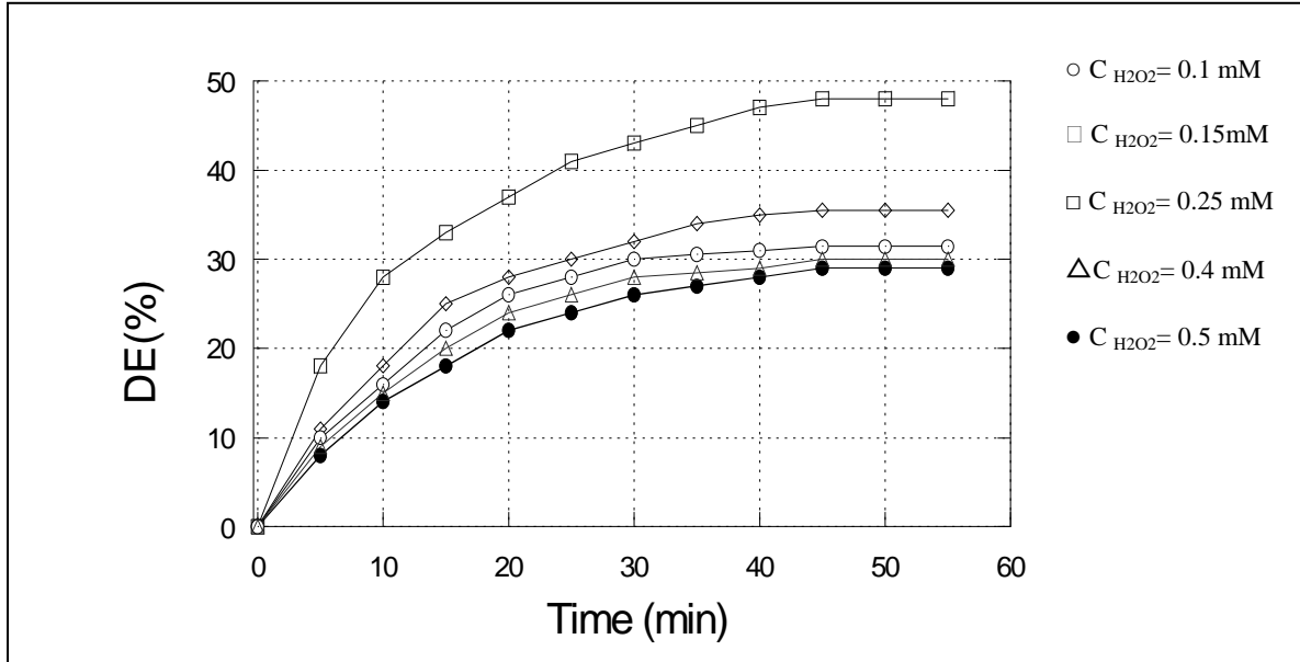
Fig.10: Effect of initial \text{H}_2\text{O}_2 concentration on MV oxidation using Cat1 as catalyst
