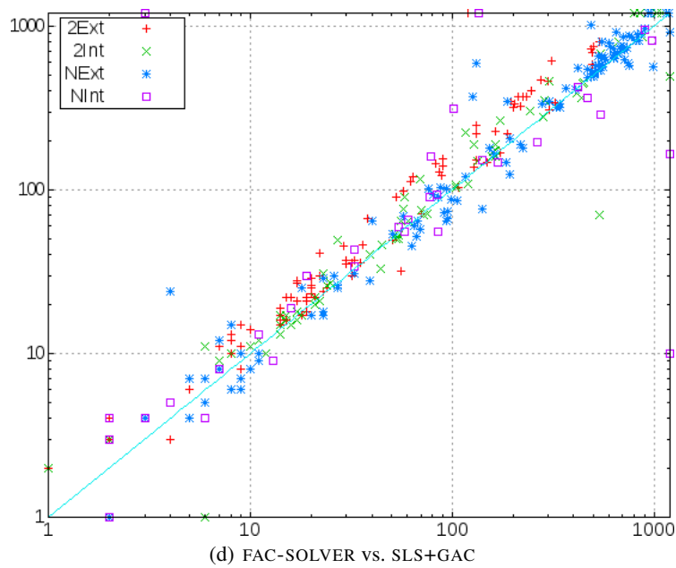
Fig. 2. Pairwise comparisons between FAC-SOLVER and classical solvers: (a) (b) (c) satisfiable instances/(d) (e) unsatisfiable instances (con't).
