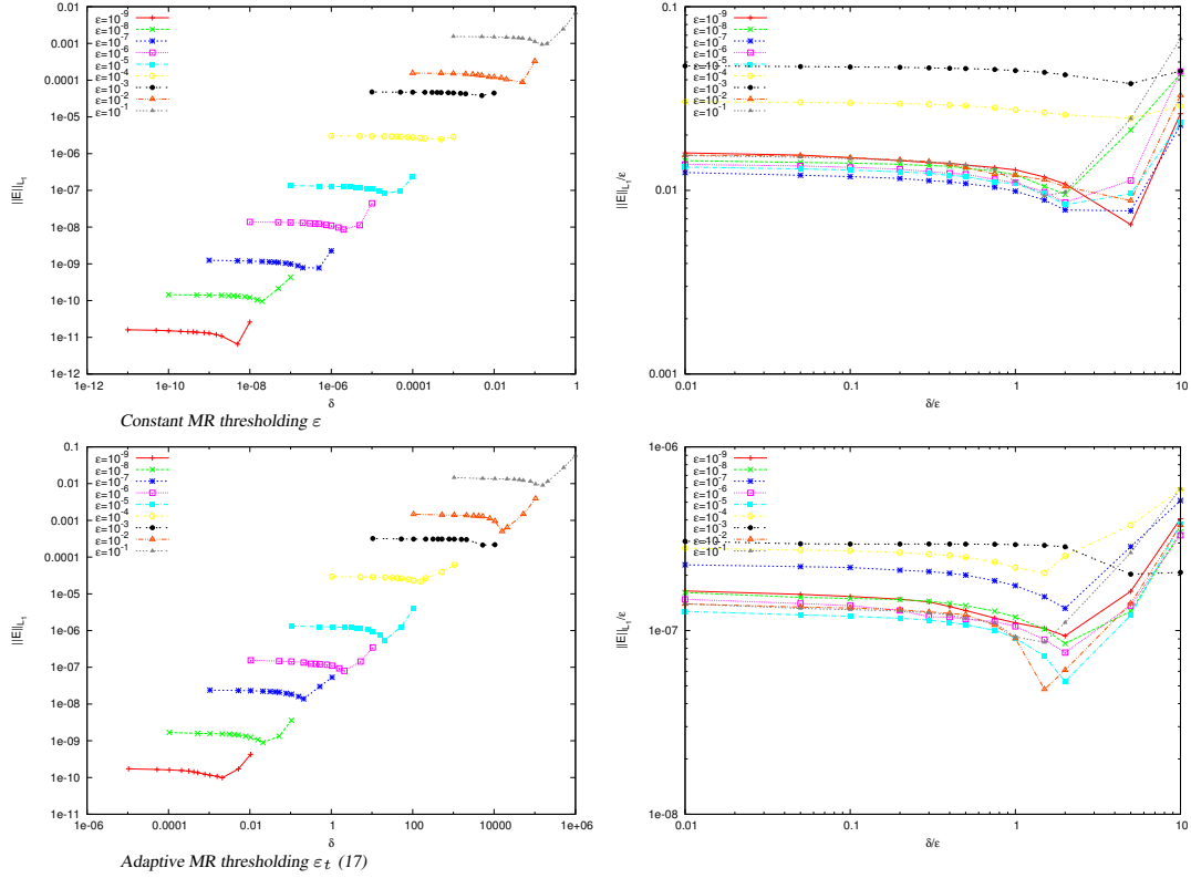
FIGURE 11. Relation between the MR threshold parameter \varepsilon and the threshold \delta in the adaptive doubling interface (18). L_1 norm of the error with the solution computed on the uniform finest grid at final time. Simple 1D test case (1), four MR levels, third order FV scheme. Left panels: error as a function of \delta . Right panels: error/ \varepsilon as a function of \delta/\varepsilon . Top panels: constant MR threshold \varepsilon , bottom panels: adaptive MR threshold \varepsilon_t
