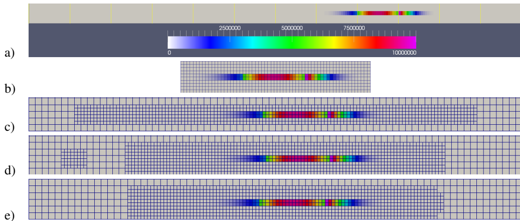
FIGURE 2. Solution at t = 20 on the whole computational domain and color code from 0 to 10^7 . Panels from top to bottom: a) finer grid no MR, b) Zoom on the support of the solution, finer grid no MR, c) MR with Haar reconstruction, d) MR with quadratic reconstruction, e) MR with quadratic reconstruction and doubling threshold strategy (18). Notice the presence (in panel d)), or absence (in panel e)) of the spurious noise
