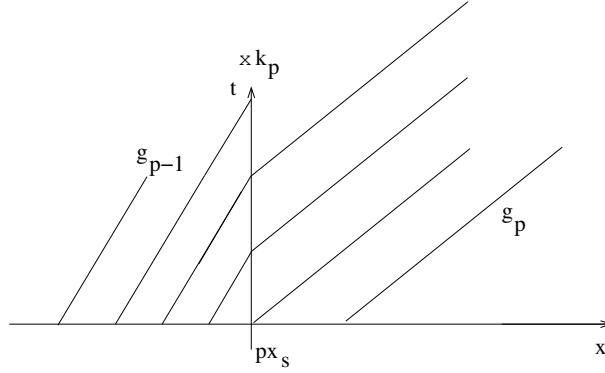
FIGURE 4. Set-up for the p^{\text{th}} interface. The characteristic curves in the right part of the domain transport either the initial condition if they cross the x -axis or the trace of the solution on the px_s interface, multiplied by the k_p coefficient, if they cross the vertical x = px_s axis
