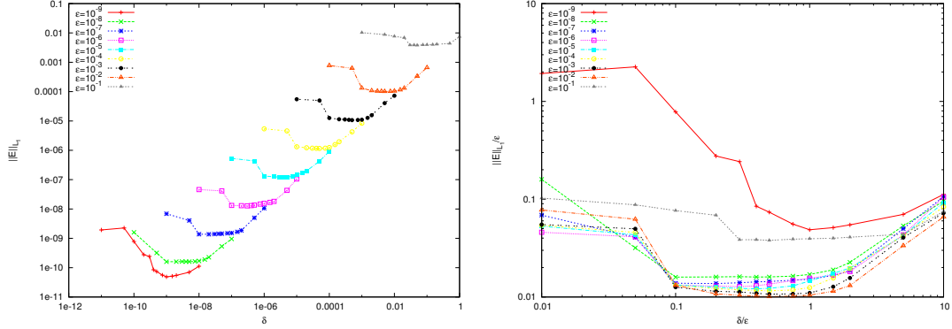
FIGURE 16. Relation between the MR threshold parameter \varepsilon and the threshold \delta in the adaptive doubling interface (18). L_1 norm of the error with the solution computed on the uniform finest grid at final time. Biological model, four MR levels, third order FV scheme. Error as a function of \delta (left), error as a function of \delta/\varepsilon , error/ \varepsilon as a function of \delta/\varepsilon , for different values of \varepsilon . Constant MR threshold \varepsilon
