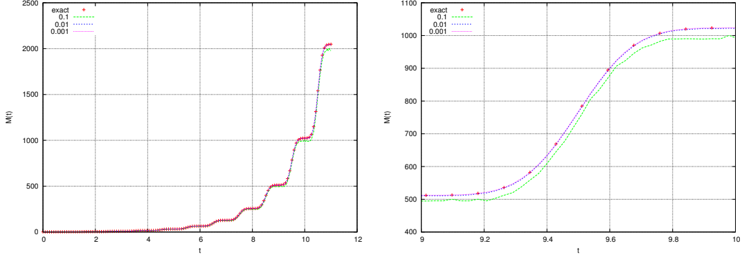
FIGURE 5. Mass with respect to time computed with the recursive definition (23), without and with the doubling strategy (18) for different values of the parameter \delta . Full time range on the left and zoom on the final region on the right
