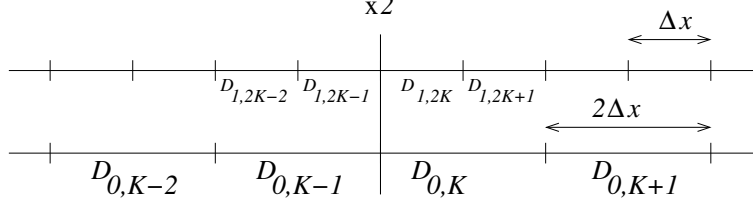
FIGURE 1. Two level discretization with doubling interface located between meshes D_{0,K-1} and D_{0,K} on the coarser level, or D_{1,2K-1} and D_{1,2K} on the finer level
