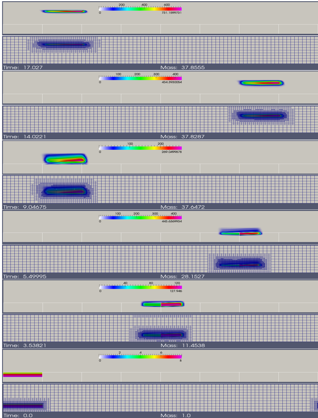
FIGURE 13. Snapshots of the density of granulosa cells computed with the FVMR strategy, adaptive doubling (18) and MR threshold (17), four MR levels, third order scheme, \varepsilon = 10^{-2} , and biological constants from Table 2. For each time, the adaptive grid is shown below the density, displayed with a time-dependent color code. The boundaries between biological cell cycles are marked with white lines
