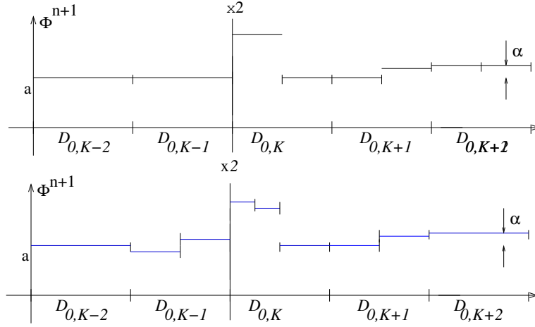
FIGURE 19. Discrete solution in example B. Top panel: updated solution at time t_{n+1} with formula (42). Bottom panel: solution computed with detail thresholding (43) according to Algorithms 1 and 2
