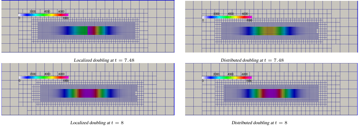
FIGURE 8. Snapshot of the solution at time t = 7.48 (top panels) and t = 8 (bottom panels). Left panels: localized doubling, right panels : distributed gain over the cell cycle
