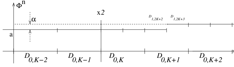
FIGURE 18. Setup for Appendix B. Three level discretization with doubling interface located between meshes \mathcal{D}_{0,K-1} and \mathcal{D}_{0,K} on the coarsest level. At time t_n the solution is piecewise constant with a discontinuity of size \alpha located between meshes \mathcal{D}_{1,2K+2} and \mathcal{D}_{1,2K+3} , resulting in a gradually adaptive grid
