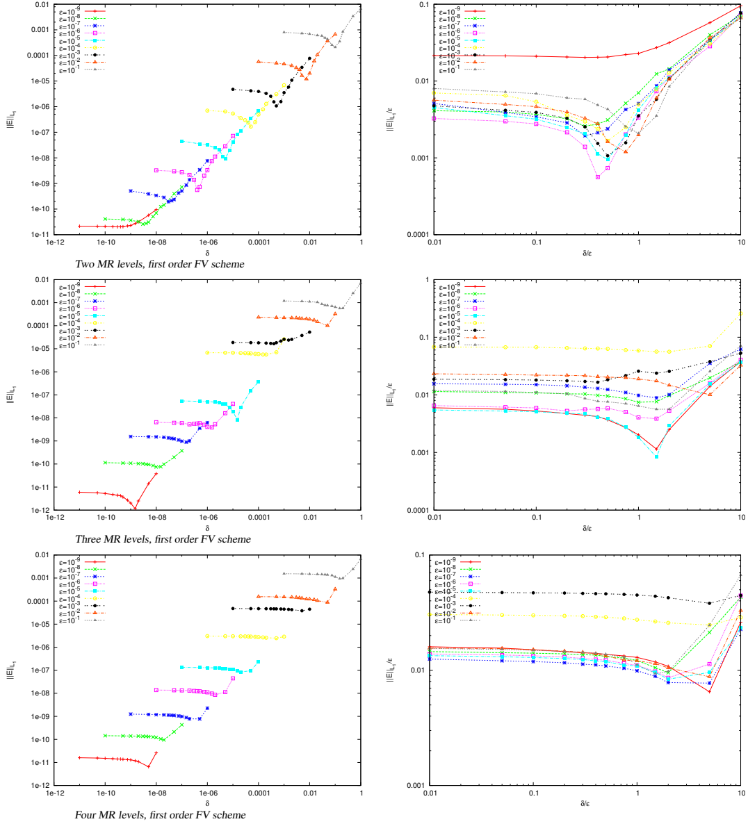
FIGURE 10. Relation between the MR threshold parameter \varepsilon and the threshold \delta in the adaptive doubling interface (18). L_1 norm of the error with the solution computed on the uniform finest grid at final time. Simple 1D test case (1) with first order FV scheme. Left panels: error as a function of \delta . Right panels: error/ \varepsilon as a function of \delta/\varepsilon , for different numbers of MR levels (top panels: L = 2 , middle panels: L = 3 , bottom panels: L = 4 )
