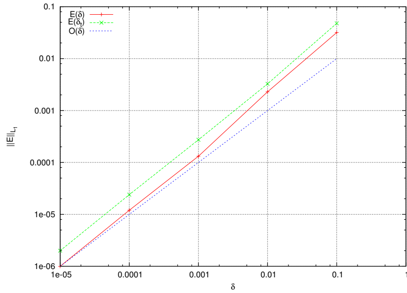
FIGURE 6. L1 norm error (27) of mass with respect to the parameter \delta of the doubling strategy (18) with ( E(\delta_i) ) and without ( E(\delta) ) time adaptivity (28). The curve O(\delta) indicates the theoretical asymptotic behavior
