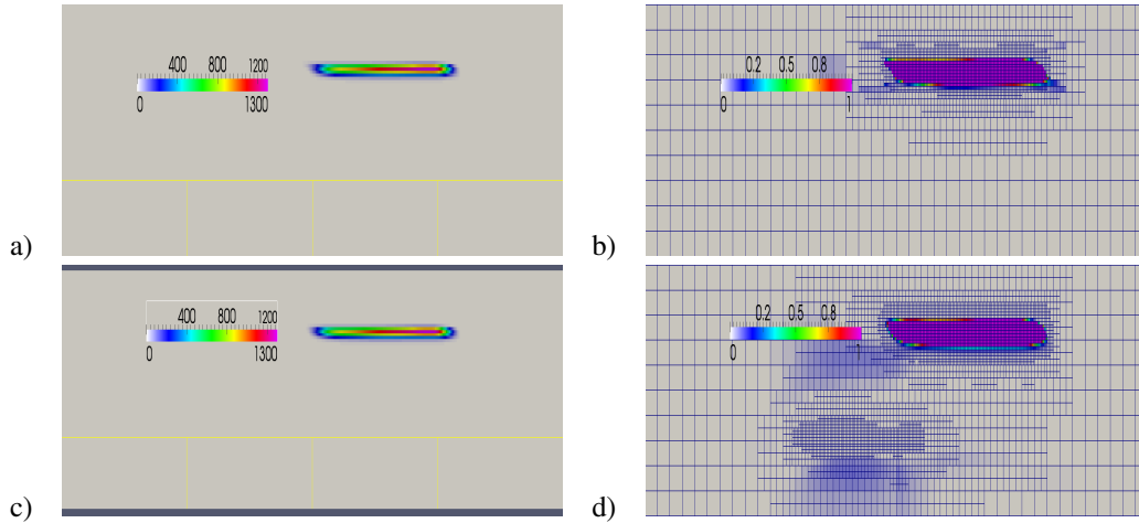
FIGURE 14. Snapshots of the density at final time t = 20 . a-b) with the adaptive doubling (18) and MR threshold strategy (17), c-d) : unconditional doubling and constant MR threshold. b-d) The color code adapted to the initial condition is used in order to highlight the spurious noise. Without the adaptive doubling strategy, the spurious noise appears and triggers additional refinement (bottom part of panel d))
