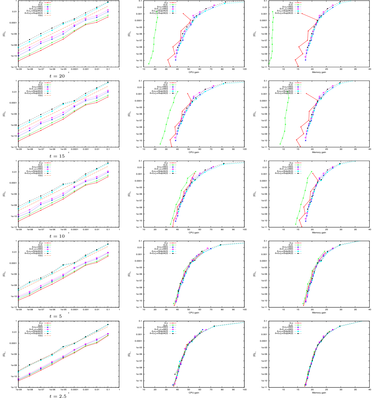
FIGURE 9. L1 norm of relative error (30) at different times, with respect to the MR threshold \epsilon (left panel), the CPU gain (center panel) and the memory gain (right panel). Effect of adaptive MR threshold \epsilon_t and doubling threshold \delta in the case of the simple 1D test case, 4 MR levels, third order FV scheme. The line labelled O(\epsilon) in the left panel graphs indicates the theoretical asymptotic behavior of the error as a function of \epsilon , the complete legend code is described in Table 1
