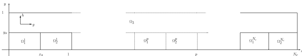
FIGURE 12. Computational domain for the biological model of follicular development. The cell cycles \Omega_1^p \cup \Omega_2^p , p = 1, \dots, N_c of unit width are periodically reproduced. \Omega_1^p corresponds to phase G1, while \Omega_2^p aggregates phases S, G2 and M of the p th cell cycle
