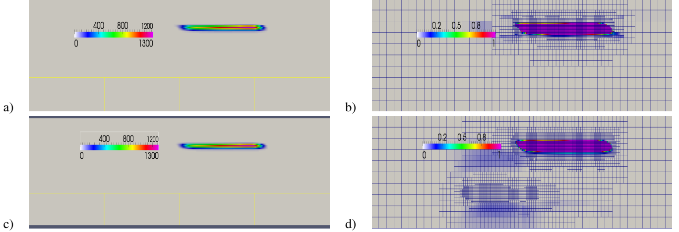
Figure 14: Snapshots of the density at final time t = 20 . a-b) with the adaptive doubling (20) and MR threshold strategy (19), c-d) : unconditional doubling and constant MR threshold. b-d) The color code adapted to the initial condition is used in order to highlight the spurious noise. Without the adaptive doubling strategy, the spurious noise appears and triggers additional refinement (bottom part of panel d)).
