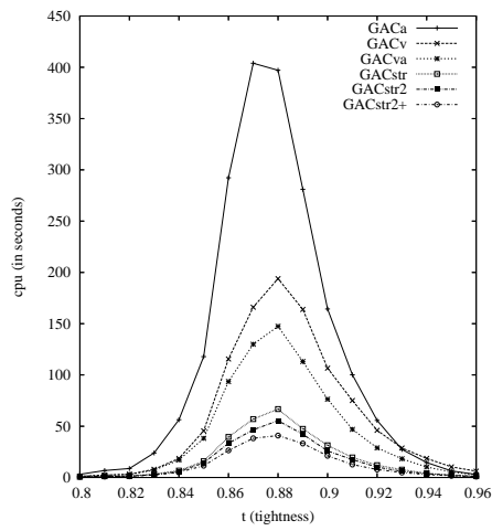
Fig. 1. Mean search cost of solving instances in classes \langle 13, 60, 2, 20, t \rangle with MAC.
