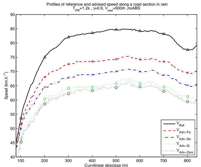
Fig. 9. Profiles of advised speeds computed with different safety criterions on wet road.
