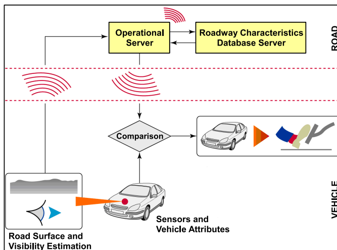
Fig. 14. Layout of Vehicle Infrastructure Integration in DIVAS Project
