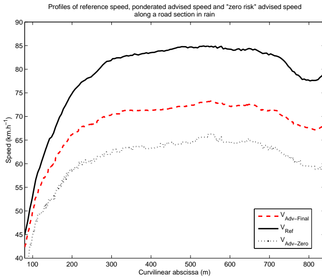
Fig. 11. Speed profiles under rainy conditions.
