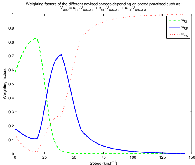
Fig. 10. Weighting of advised speeds linked to different severity levels.
