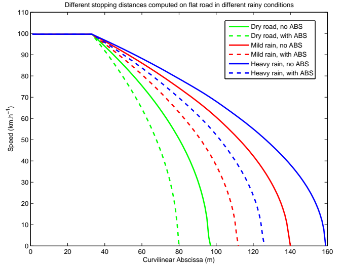
Fig. 2. Emergency braking speed profiles under various rainy conditions.
