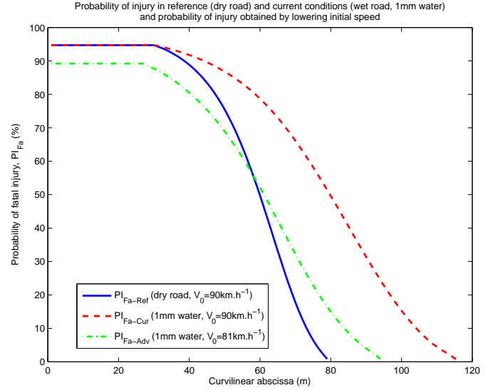
Fig. 4. Probability of fatal injury PI_{Fa} for emergency braking on wet pavement at 90 \text{ km.h}^{-1} .
