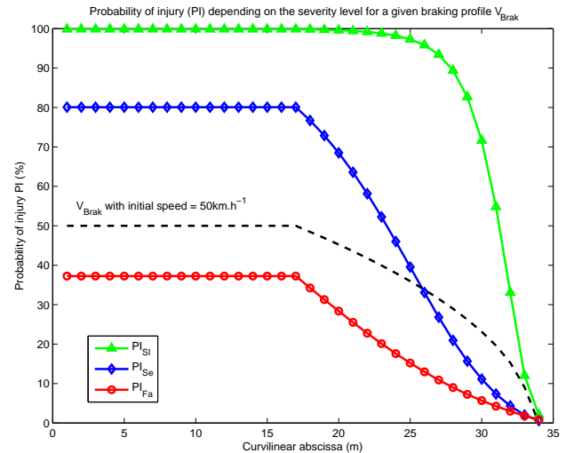
Fig. 3. Braking speed profile V_{Brak} with parameters ( V_0 = 50 km.h^{-1} , t_{PR} = 1.2s , \mu(x) = \mu_{dry}(x) \in [0.8, 0.9] , \gamma = 0.9 ) and corresponding curves of probability of injury PI_{Sl} , PI_{Se} , PI_{Fa} .
