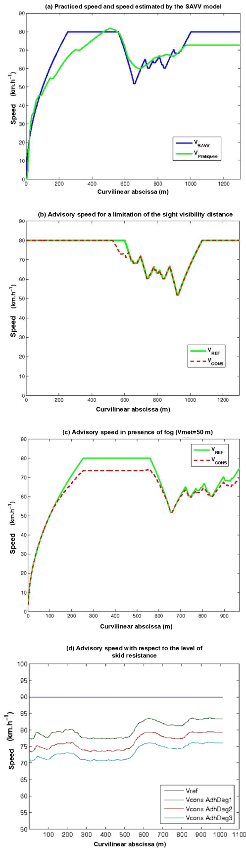
Fig. 16. Speed recommendation issued by the DIVAS system on the different test scenarios: (a) speed profile in curve; (b) speed profile in case of reduced sight distance; (c) speed profile in case of reduced meteorological visibility; (d) speed profile in case of a wet road (with different levels of skid resistance).
