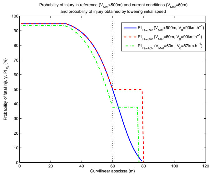
Fig. 6. Braking speed profile and probability of fatal injury in fog with 60m of visibility distance.
