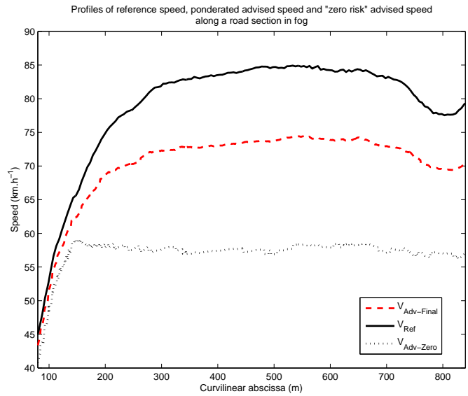
Fig. 13. Reference, "zero risk" and ETR speed profiles in fog with V_{Met} = 50 m.
