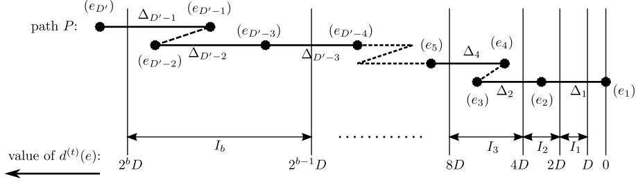
Figure 1: An illustration of sets I_i and \Delta_l in the proof of Theorem 3.3.
