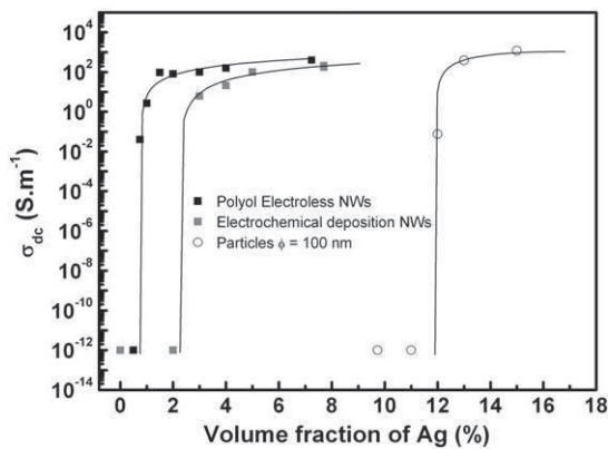
Fig. 4. Dependence of the dc conductivity ( \sigma_{dc} ) on the silver volume fraction in P(VDF-TrFE) matrix at 25 °C as a function of particles geometry: Polyol reduction process nanowires (■), Electrochemical deposited nanowires (■), 100 nm particles (○).
