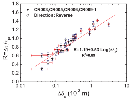
Figure 7. Semi-logarithmic plot of shear stress release level R versus imposed reverse offset \Delta\delta_c (in mm): (▼) CR003, CR005, CR006 and Phase 1 of CR009 and (◇) for a reverse direction (Direction: Reverse, in the legend) of a separate test. The red line is a logarithmic fit: R = 1.19 + 0.53 \log(\Delta\delta_c) .
