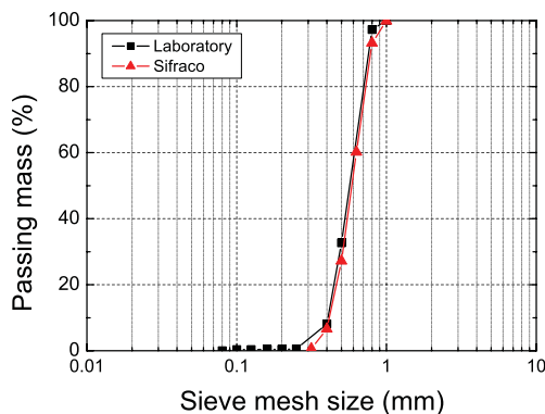
Figure 4. Grain-size distribution of the Hostun (HN; 0.4/0.8) sand from supplier data (SIFRACO) and our own laboratory check with a laser granulometer.
