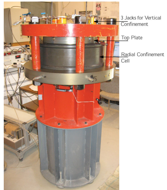
Figure 1. View of the Cylinder Shear Apparatus (ACSA).
