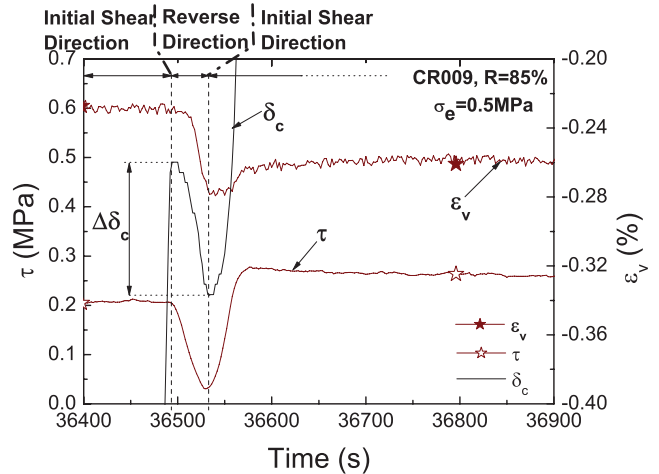
Figure 12. Detail of data acquisition at the third release sequence ( R = 85 per cent) of CR009 illustrating the shear stress (★) response measured by the torque meter and volumetric strain (★) recorded by the volume/pressure controller (which measures the total sample volume across the confinement water variation), after 3 m of cumulative slip \delta_c (line). Displacement is measured by the cylinder rotation encoder, and corresponds to the displacement at the interface steel/sample. The reverse offset undergone for the 85 per cent release is about 0.34 \cdot 10^{-3} \text{ m} .
