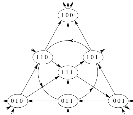
FIGURE 1. (\mathbb{Z}_2)^3 -grading on the octonions.
