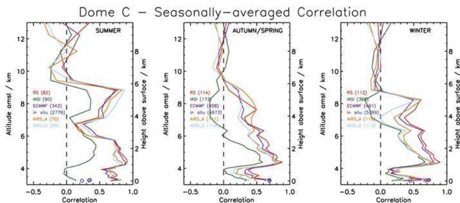
Fig. 13. As Fig. 11 but for H 2 O correlation of H 2 O Antarctica Microwave Stratospheric and Tropospheric Radiometer (HAMSTRAD) vs all the other datasets in temporal coincidence within a 60-min window.
