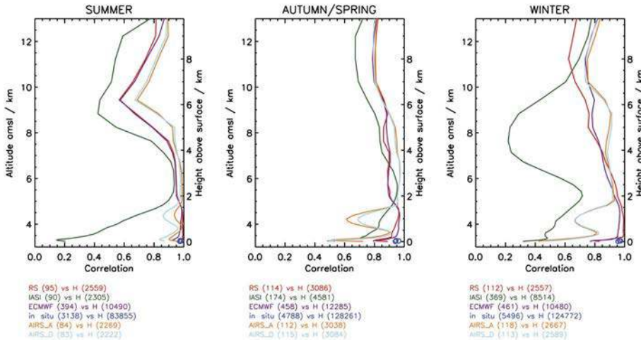
Fig. 5. As Fig. 2 but for correlation of H 2 O Antarctica Microwave Stratospheric and Tropospheric Radiometer (HAMSTRAD) temperatures vs all the other datasets in temporal coincidence within a 60-min window.
