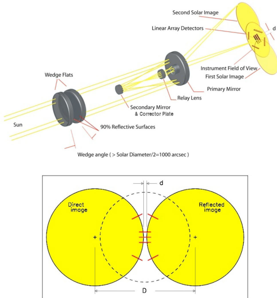
Figure 1. Upper: optical layout of the SDS. The SDS is built around a ruggedized Questar telescope supplemented with a beam splitting wedge and a Barlow relay lens to increase the focal length. The beam splitting wedge produces a direct image and a reflected image that is offset by slightly more than the Sun's diameter. The solar limb is measured along 10 radials by seven linear-array CCDs mounted in the focal plane. Insert: detail of the detector plane. The red line segments indicate the location of the CCDs; the dotted circle shows the approximate field of view. The solar diameter is determined by precise measurement of the discs' separation, D , and gap, d .
