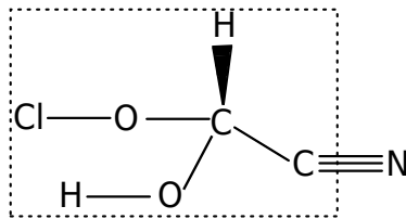
Fig. 1. Molecule with one asymmetric carbon. Its minimal chiral subtree is surrounded by dotted line.
