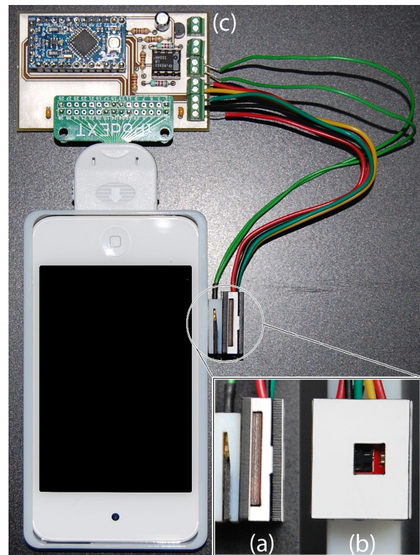
Figure 2. Our prototype, equipped with a button for sensing pressure and proximity. The sensors are placed inside custom-built plastic casings. (a) Side view of the pressure and proximity sensors. (b) Front view of the window above the proximity sensor. (c) Circuit board.
