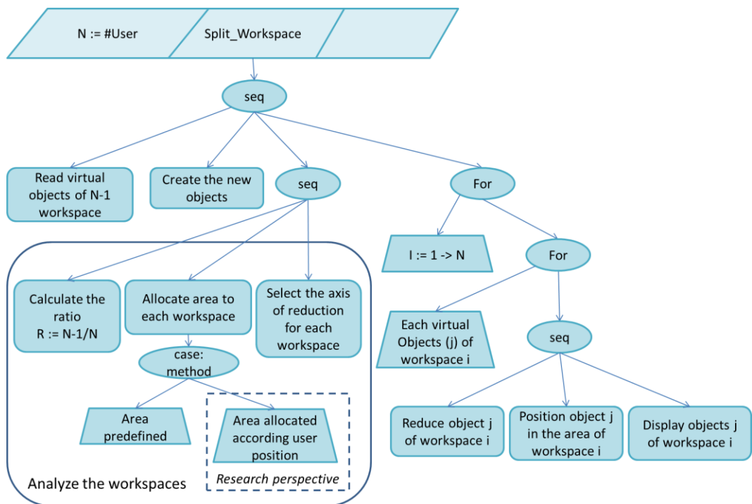
Figure 6 Split_workspace algorithm
