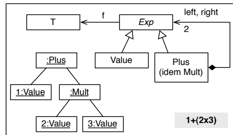
Fig. 6. Models of arithmetic expressions.
