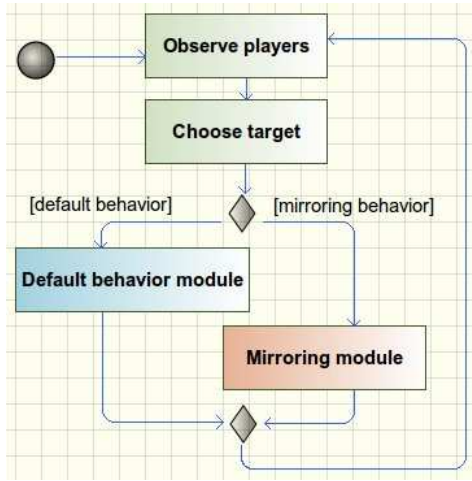
Fig. 2. Overview of MirrorBot's behavior
