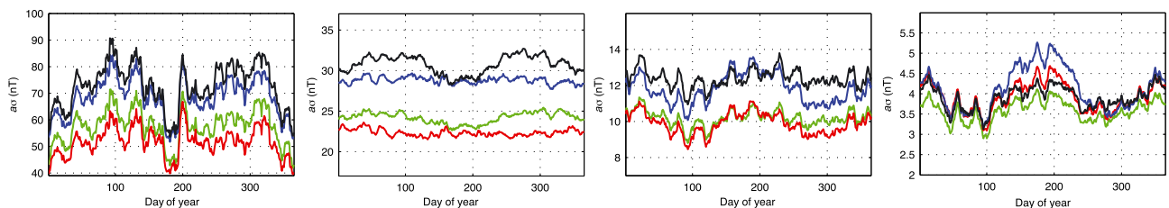
Figure 4. Comparison of the MLT sector indices separated in four activity classes, from left to right: am > 40 nT, 20 \text{ nT} < am < 40 nT, 10 \text{ nT} < am < 20 nT, and am < 10 nT. The color code is similar to that of Figure 3.
