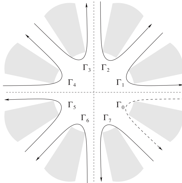
FIG. 1. Wedge and antiwedge contours for V_2(y) of degree d_2+1 ( =8 in this example).
