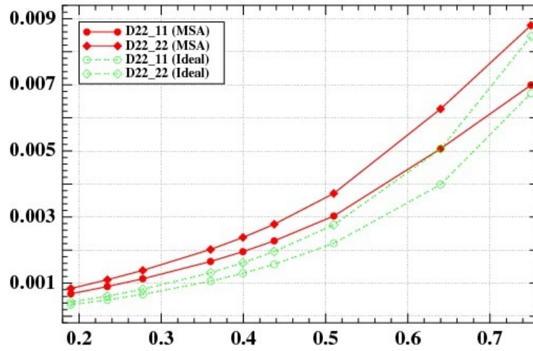
Figure 14: Electrodiffusion tensor \mathbb{D}_{22} for the anion versus porosity ( n_j^*(\infty) = 0.1\text{mole/l} )
