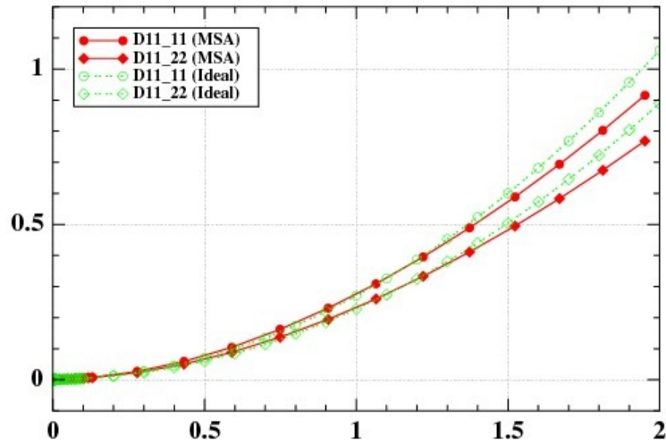
Figure 5: Entries of the electrodiffusion tensor \mathbb{D}_{11} for the cation, as functions of the dimensional (mol/l) infinite dilution concentrations n_j^*(\infty)
