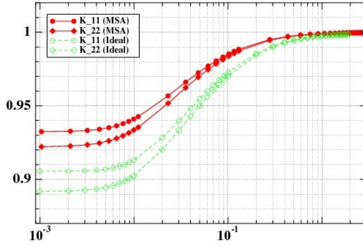
Figure 4: Diagonal entries of the relative permeability tensor, \mathbb{K}_{11} and \mathbb{K}_{22} , as functions of the dimensional (mol/l) infinite dilution concentrations n_j^*(\infty)
