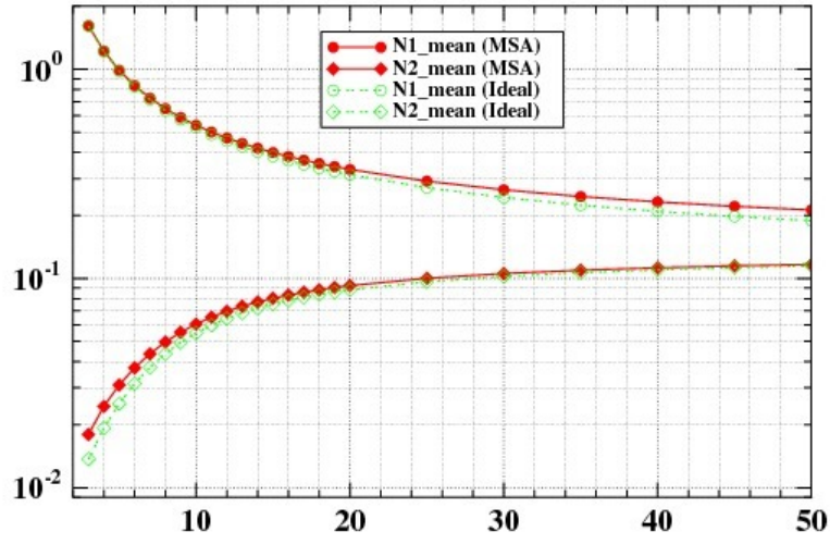
Figure 9: Averaged cell concentration N_{j\_mean} = |Y_F|^{-1} \int_{Y_F} n_j(y) dy versus pore size \ell (nm)
