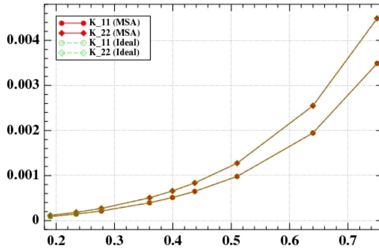
Figure 12: Permeability tensor \mathbb{K} versus porosity ( n_j^*(\infty) = 0.1 \text{mole/l} )
