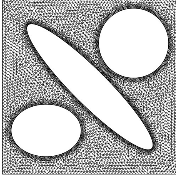
Figure 1: Mesh for a periodicity cell with ellipsoidal inclusions (porosity is equal to 0.62)
