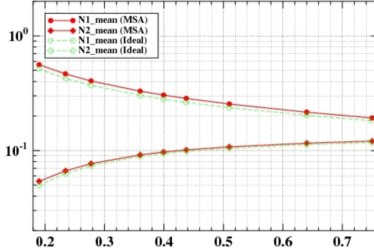
Figure 11: Averaged cell concentration N_{j\_mean} = |Y_F|^{-1} \int_{Y_F} n_j(y) dy versus porosity ( n_j^*(\infty) = 0.1 \text{mole/l} )
