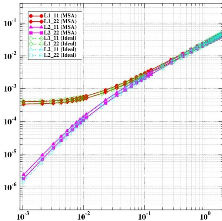
Figure 8: Diagonal entries of the coupling tensors \mathbb{L}_1 and \mathbb{L}_2 , as functions of the dimensional (mol/l) infinite dilution concentrations n_j^*(\infty) (log-log plot)
