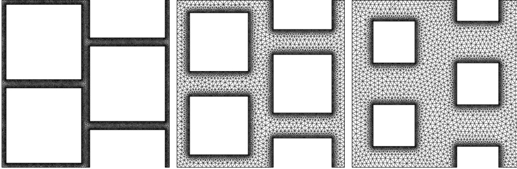
Figure 2: Meshes for three different porosities (0.19, 0.51 and 0.75) of a periodic cell with rectangular inclusions
