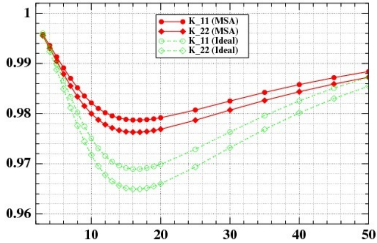
Figure 10: Relative permeability coefficients \mathbb{K}_{11} and \mathbb{K}_{22} versus pore size \ell (nm)
