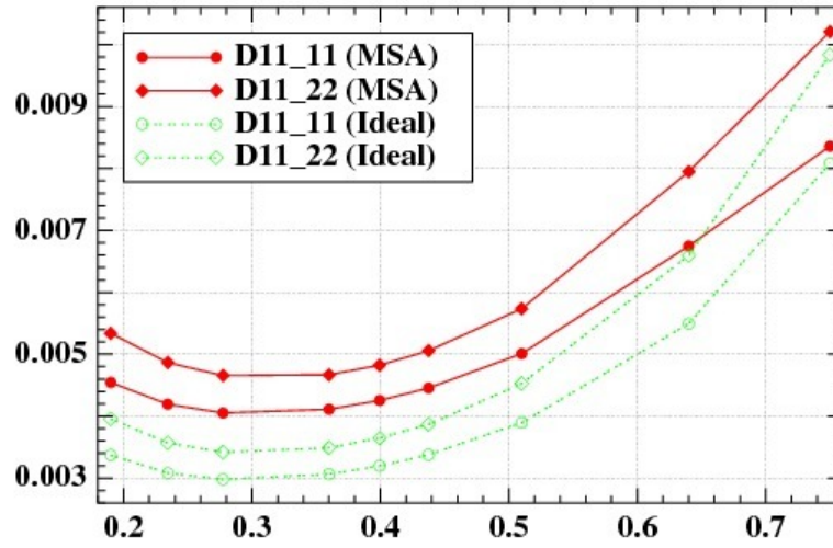
Figure 13: Electrodiffusion tensor \mathbb{D}_{11} for the cation versus porosity ( n_j^*(\infty) = 0.1\text{mole/l} )
