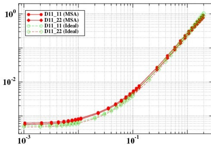
Figure 7: Diagonal entries of the electrodiffusion tensor \mathbb{D}_{11} as functions of the dimensional (mol/l) infinite dilution concentrations n_j^*(\infty) (log-log plot)
