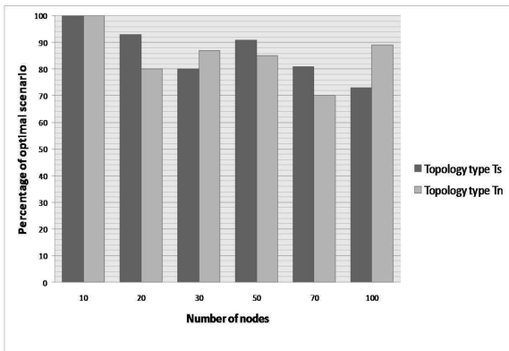
Fig. 3. Optimality of MODESA in T_S and T_N configurations.
