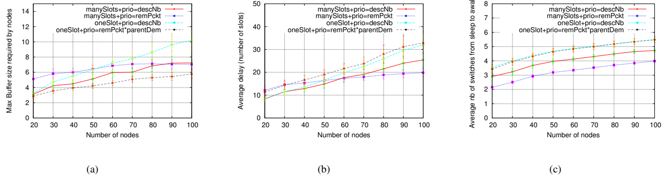
Fig. 3. TRASA performance regarding (a) Maximum buffer size (b) Average delay (c) Number of radio switches.
