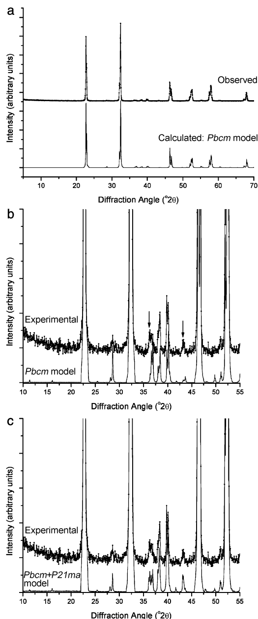
Fig. 2 Powder X-ray diffraction data from hydrothermal \text{NaNbO}_3 (a) compared to data calculated from the Pbcm model, (b) an expanded area with arrows indicating additional intensity not predicted by the Pbcm model and (c) compared to data calculated from a model with a mixture of two polymorphs.
