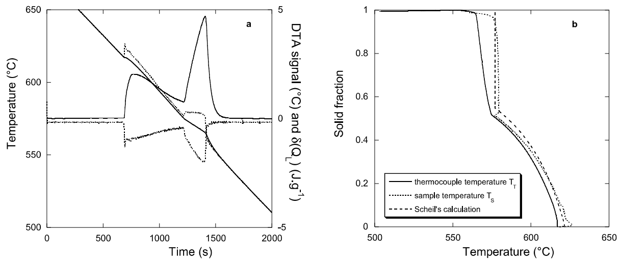
Figure 4 – (a) Reverse calculation applied to solidification at 5 \text{ K}/\text{min} of an Al-Si alloy; the calculated T_S and \delta(Q_L) values are showed with dotted lines while the input T_T and \Delta T curves are in solid lines.
