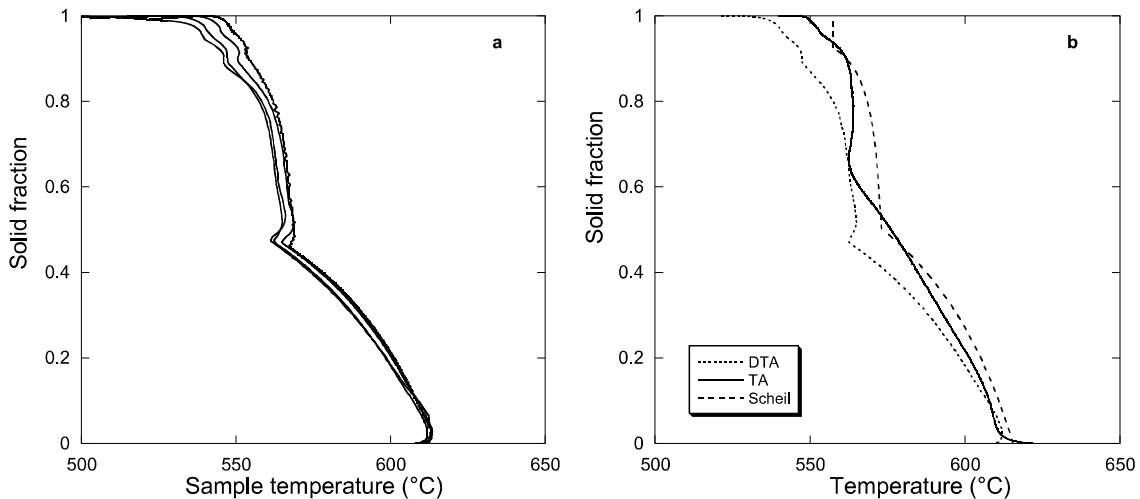
Figure 5 – (a) Solidification kinetics calculated from DTA records at increasing cooling rate (5, 10, 15 and 20 K.min -1 ) on AS7G samples; (b) comparison of the solidification kinetics estimated from TA and DTA (15 K.min -1 ) as compared to thermodynamic prediction.
