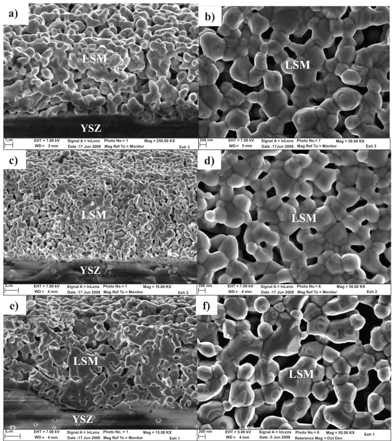
Fig. (3). SEM micrographs relative to surface morphology and cross-section of (a, b) YSZ/YSZ(dip-coating)/LSM (c, d) YSZ/YSZ(PVD)/LSM and e,f) YSZ/YSZ(ALD)/LSM samples.
