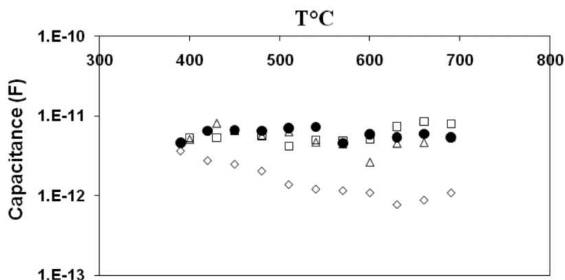
Fig. (11). Plots of the capacitance of the electrolyte response (HF) for \Delta ) YSZ/YSZ(PVD)/LSM, \square ) YSZ/YSZ(dip-coating)/LSM, \diamond ) YSZ/YSZ(ALD)/LSM and \bullet ) YSZ/Pt.
