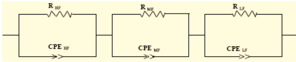
Fig. (8). Equivalent circuit used for fitting Impedance diagrams of samples.
