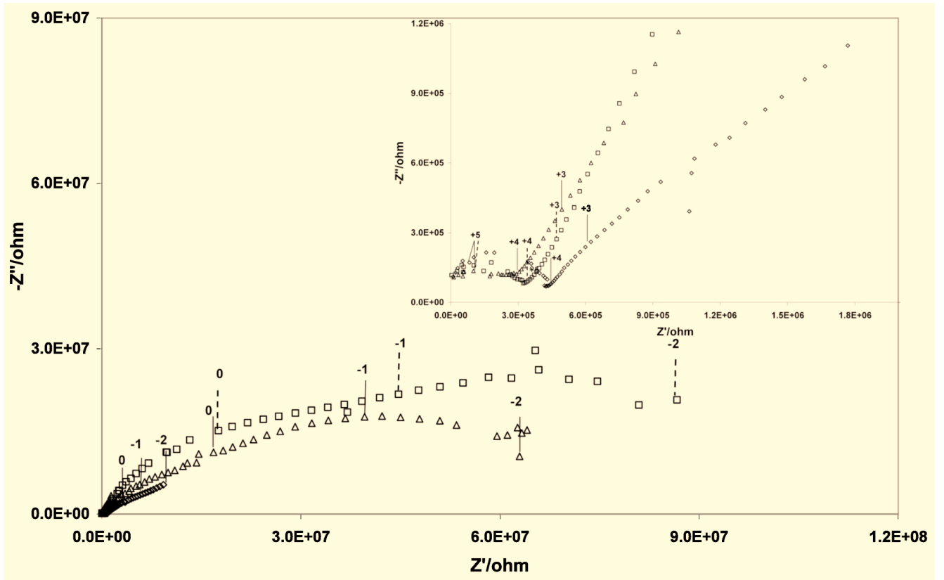
Fig. (6). Impedance diagrams measured at 450 °C for \Delta )YSZ/YSZ (PVD)/LSM, \square )YSZ/YSZ(dip-coating)/LSM and \diamond )YSZ/YSZ (ALD)/LSM. Frequency logarithms are indicated.
