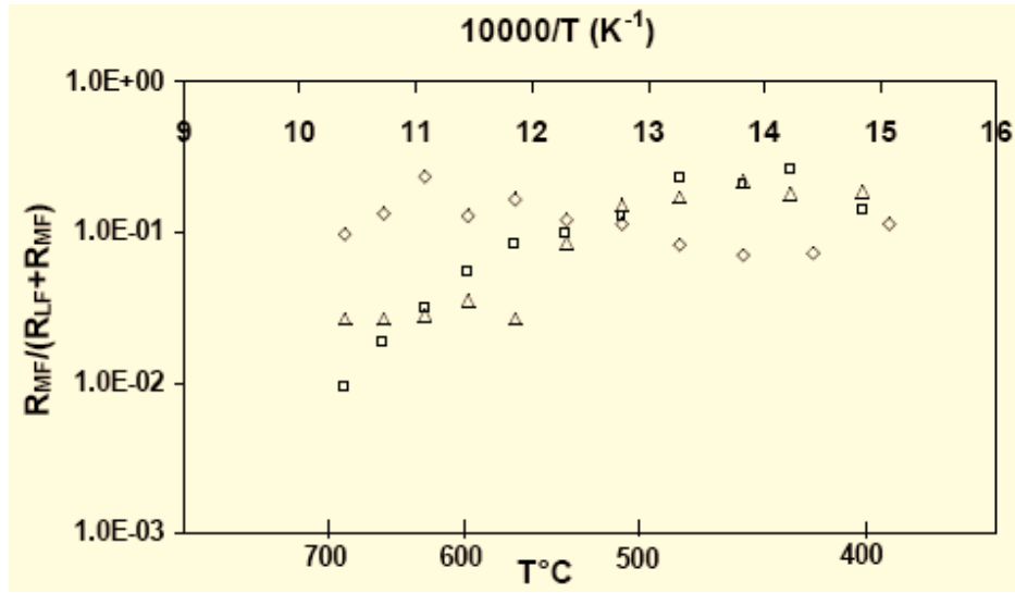
Fig. (12). Plots of the ratio ( R_{MF}/(R_{MF}+R_{LF}) ) versus the temperature (HF) for \Delta ) YSZ/YSZ(PVD)/LSM, \square ) YSZ/YSZ(dip-coating)/LSM and \diamond ) YSZ/YSZ(ALD)/LSM.
