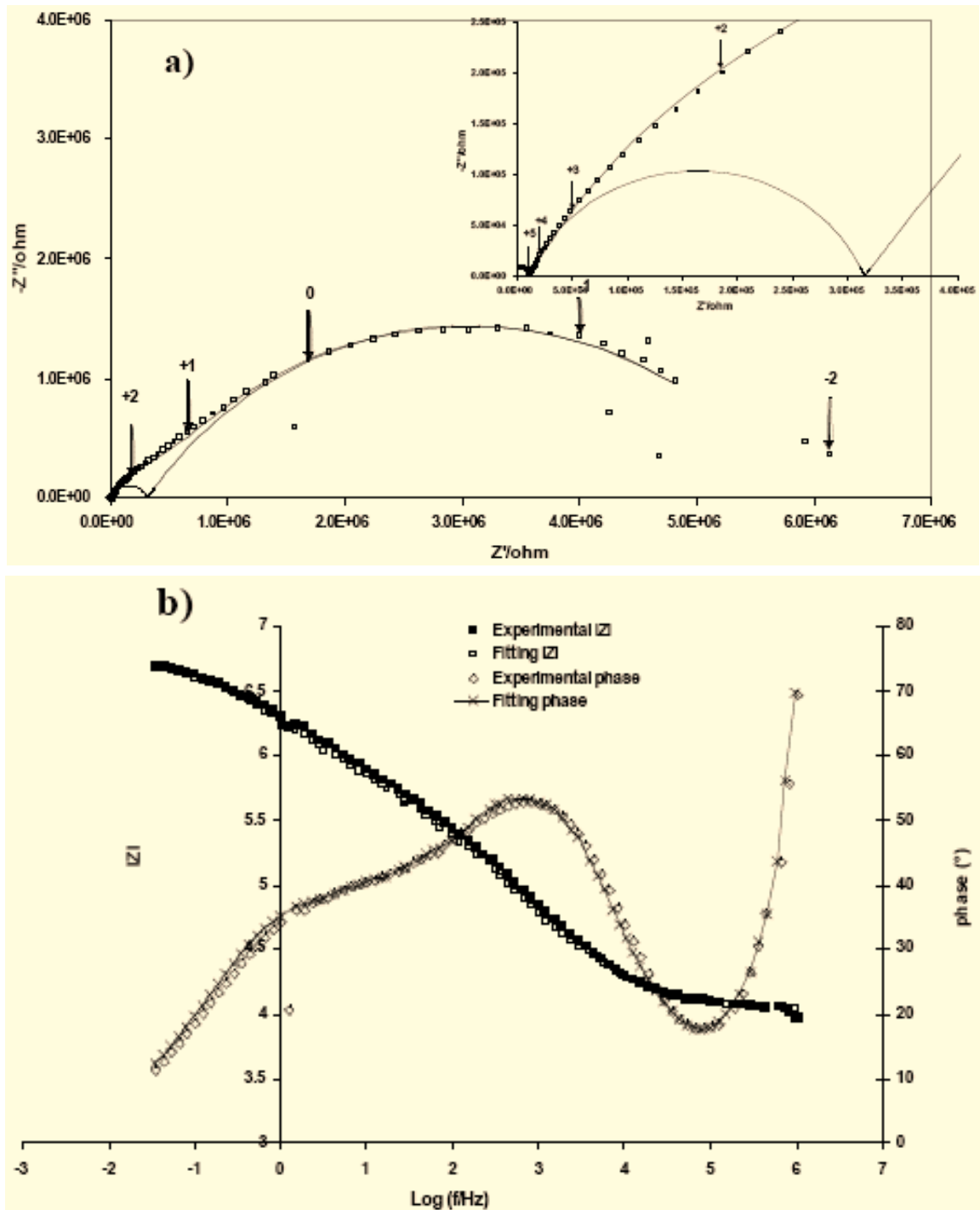
Fig. (9). Fitted results of experimental data measured at 600 °C for YSZ/YSZ(dip-coating)/LSM sample. (□) Experimental data; lines are the fitted results (a) Nyquist diagram and (b) Bode diagram.
