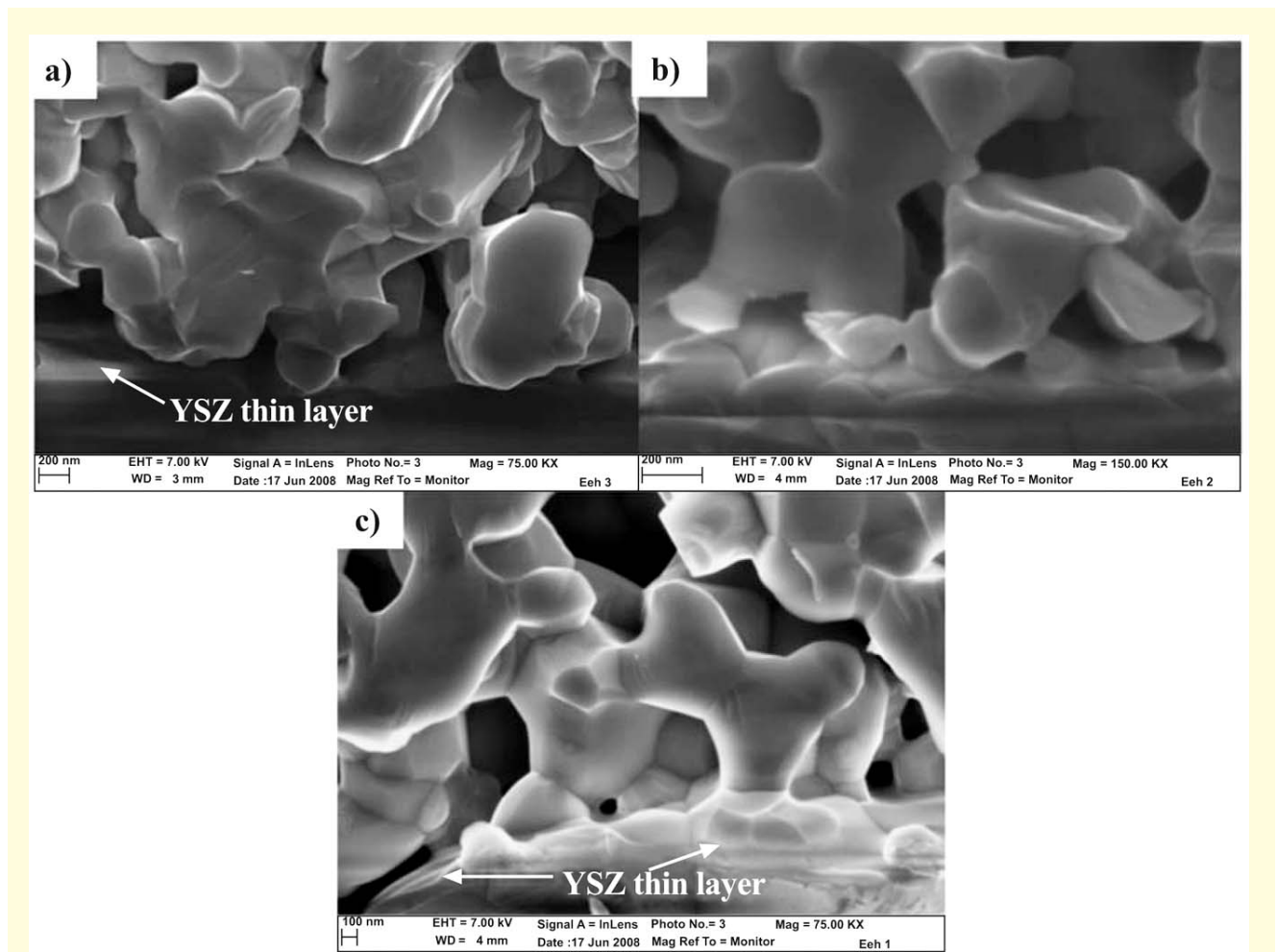
Fig. (5). SEM micrographs of the cross-sections of (a) YSZ/YSZ(dip-coating)/LSM (b) YSZ/YSZ(PVD)/LSM and (c) YSZ/YSZ(ALD)/LSM samples.
