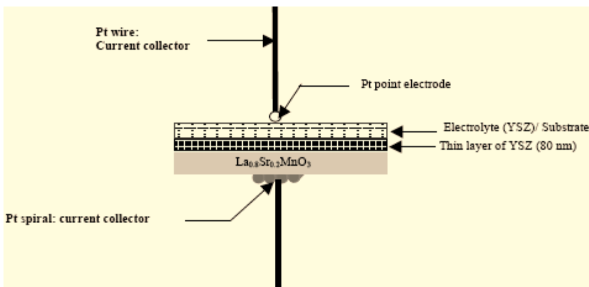
Fig. (2). Scheme of the measurement device used for the impedance spectroscopy measurements [4].
