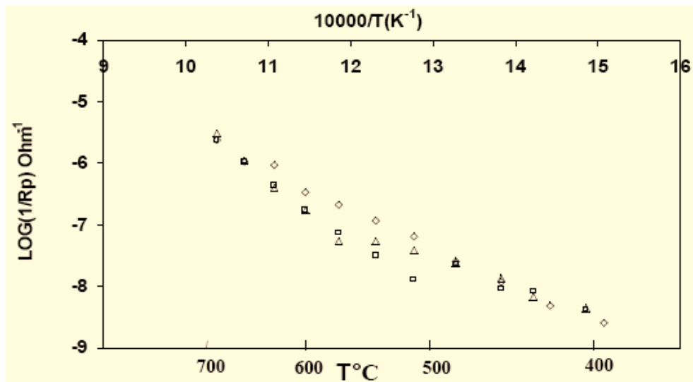
Fig. (13). Arrhenius plots of the polarisation resistance for \Delta ) YSZ/YSZ(PVD)/LSM, \square ) YSZ/YSZ(dip-coating)/LSM and \diamond ) YSZ/YSZ(ALD)/LSM.
