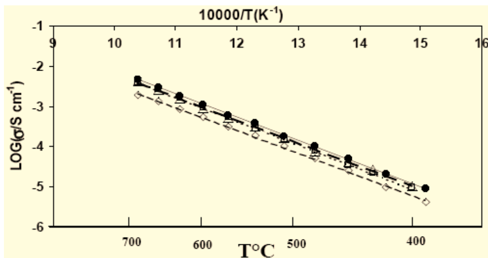
Fig. (10). Arrhenius plots of the electrolyte conductivity (HF) for \Delta ) YSZ/YSZ(PVD)/LSM, \square ) YSZ/YSZ(dip-coating)/LSM, \diamond ) YSZ/YSZ(ALD)/LSM and \bullet ) YSZ/Pt.
