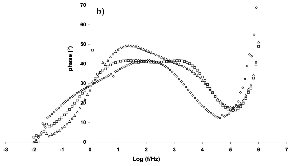
Fig. (7). Impedance diagrams measured at 660 °C for \Delta )YSZ/YSZ (PVD)/LSM, \square )YSZ/YSZ(dip-coating)/LSM and \diamond )YSZ/YSZ(ALD)/LSM. a) Nyquist diagram (frequency logarithms are indicated), b) Bode diagram.
