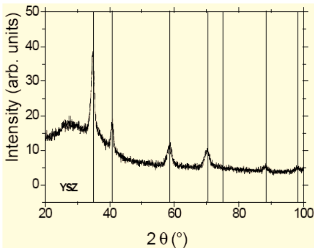
Fig. (4). X-ray diffractogram of an 80 nm YSZ layer deposited on soda-lime glass substrate. The vertical lines represent the theoretical positions of the YSZ diffraction peaks.
