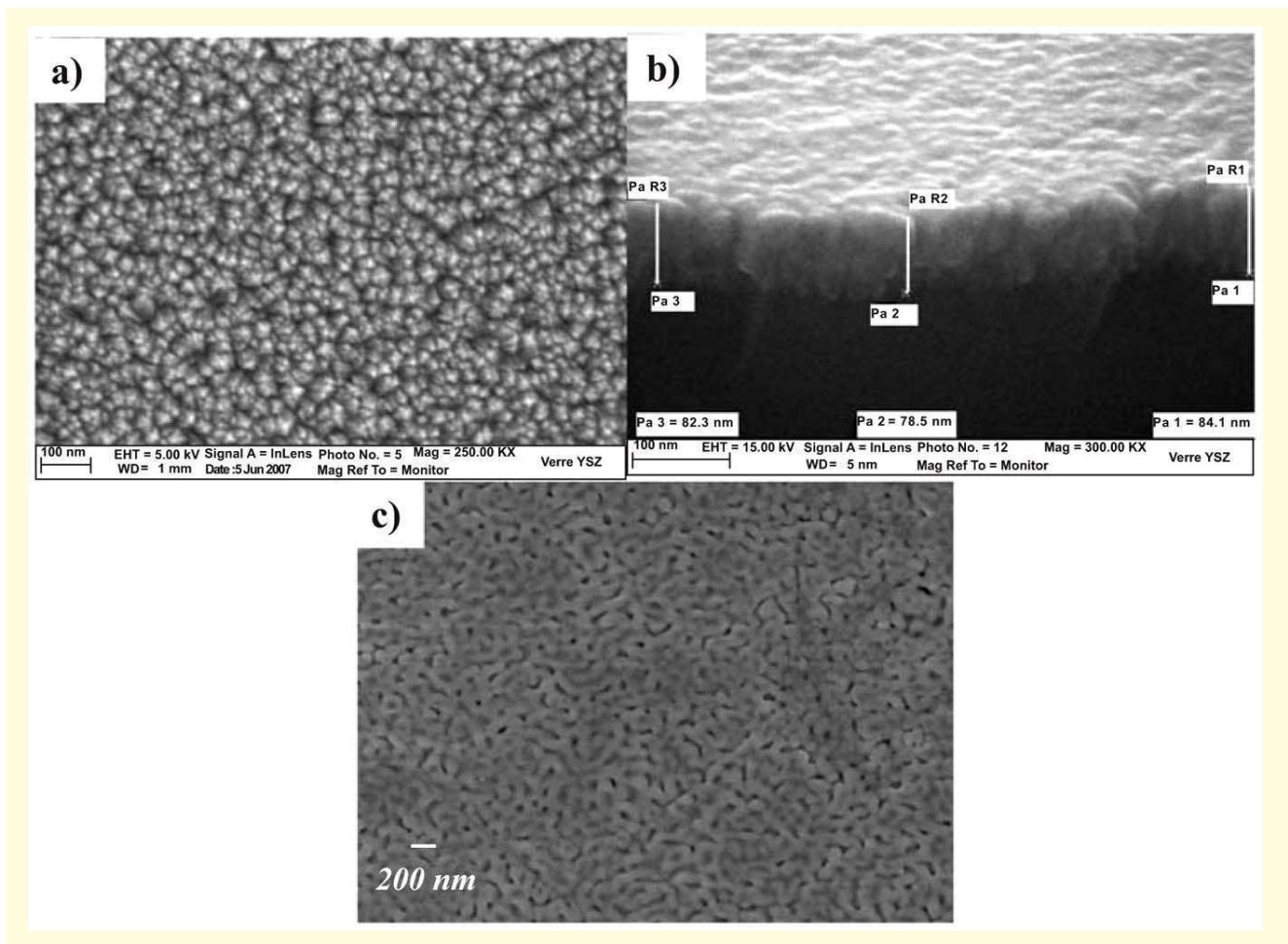
Fig. (1). SEM micrographs relative to YSZ thin layers deposited by ALD onto soda-lime glass (a) surface morphology, (b) cross-section and (c) surface morphology deposited by dip-coating onto YSZ substrate.
