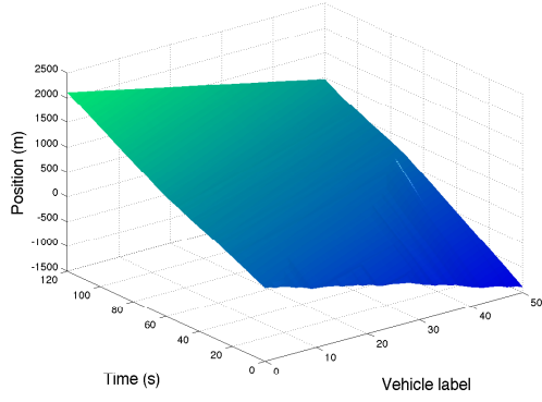
(a) Moskowitz surface X(t, n)
