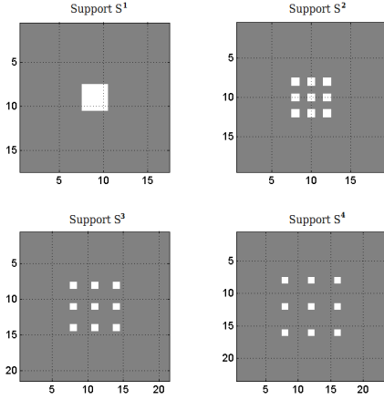
Fig. 1: The supports \text{rg}(S^k) described by (15), for d=2 , k \in \{1, 2, 3, 4\} and for c=1 (i.e., S=3 \times 3 ). The representation is shifted so that the origin element of (15) is at the center of each image. The constraint (2) forces each kernel h^k to take the value 0 outside of \text{rg}(S^k) .
