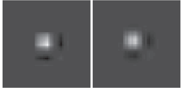
Fig. 21 Estimation of the low frequency wavelet atom at level 3. Atom H ( left ) and \lambda \alpha * h^1 * \dots * h^K ( right ). \text{PSNR}_H = 29.94
