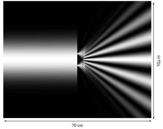
FIG. 2. General view of the evolution of the probability density from the source to the screen in the Jönsson experiment. A lighter shade means that the density is higher i.e. the probability of presence is high.
