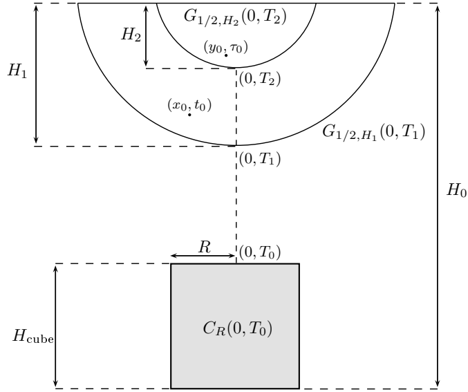
FIGURE 2. Geometry in the proof of Proposition 3.1: the cube C_R(0, T_0) and the parabolic balls G_{1/2, H_1}(0, T_1) and G_{1/2, H_2}(0, T_2) such that C_R(0, T_0) \subseteq G_{\theta, H_0}^-(x_0, t_0) with (x_0, t_0) \in G_{1/2, H_1}(0, T_1) .
