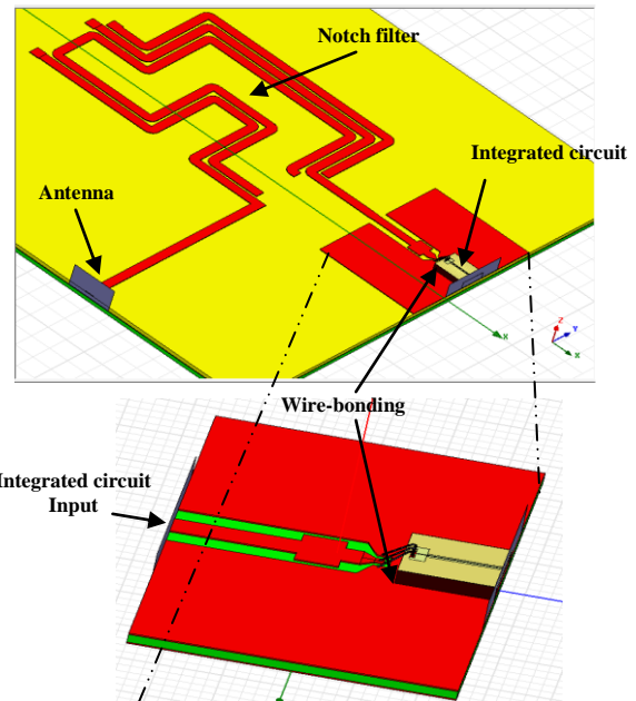
Fig. 8. Two-paths notch filter connected to the IC chip using wire-bonding.
