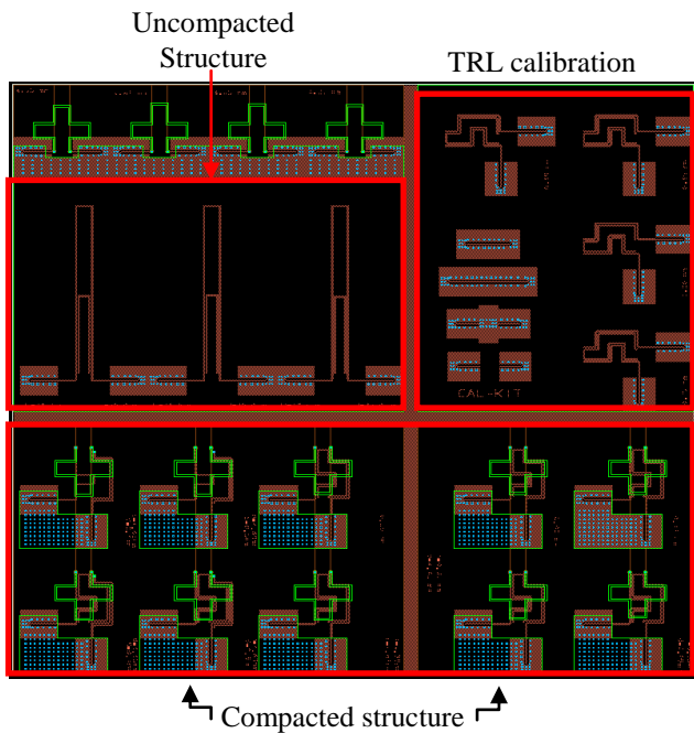
Fig. 10. Layout of the two-path notch filter.
