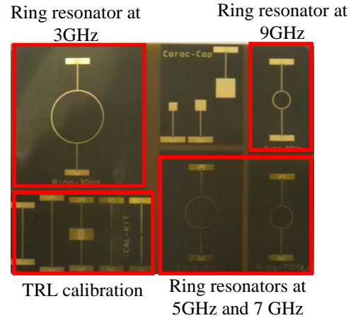
Fig. 2. Fabricated ring resonators on 125 \mu\text{m} Kapton-based substrate.
