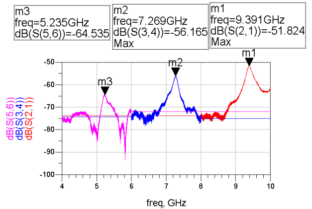
Fig. 3. S21 vs. frequency for three ring resonators.
