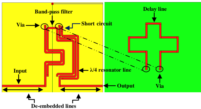
Fig. 5. Two-paths notch filter concept.
