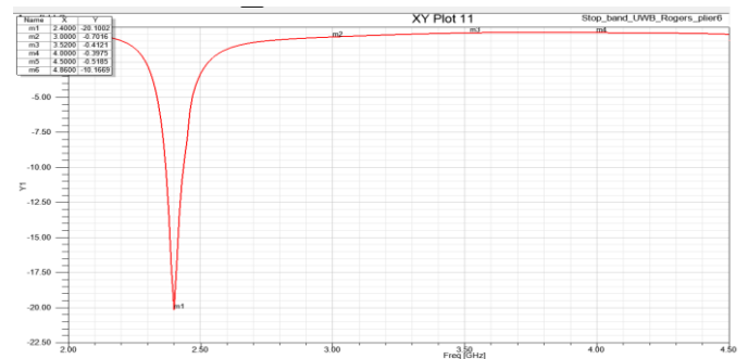
Fig. 7. Simulated S_{21} of the filter VS frequency.
