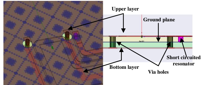
Fig. 6. Cross-view of the compacted two-path notch filter.
