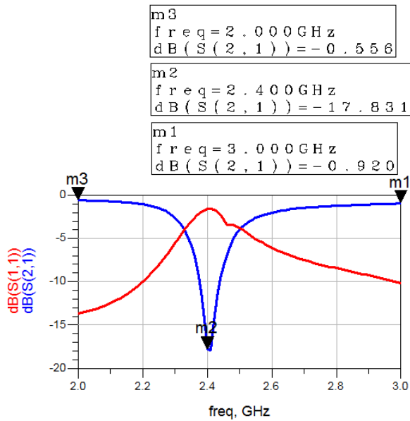
Fig. 9. Simulated S21 of the complete structure VS frequency.
