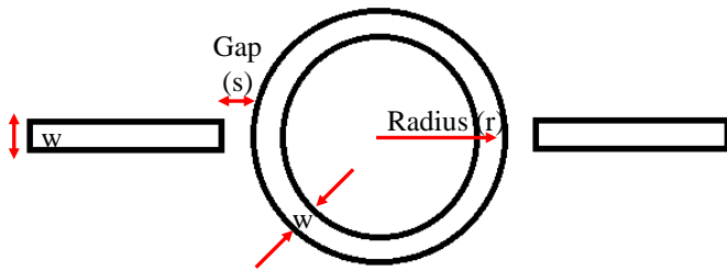
Fig. 1. Microstrip ring resonator configuration diagram.
