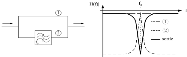
Fig. 4. Two-path notch filter concept.
