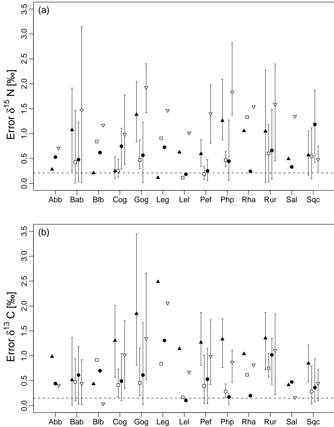
Figure 3: Mean values of the four types of errors for each species for \delta^{15}\text{N} values (3a) and for \delta^{13}\text{C} values (3b). Black up-triangles, white squares, black circles and white down-triangles corresponds to E, ES, EG and EJ, respectively. Vertical bars give the range between minimum and maximum values. Horizontal dashed line indicates the level of analytical precision.
