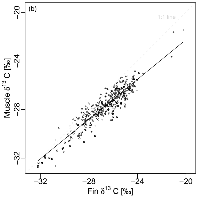
Figure 2: Linear models (black segment) between muscle and fin \delta^{15}\text{N} values (2a) or fin \delta^{13}\text{C} values (2b), constructed with all 1416 fish (+ = cyprinidae, o = percidae, x = Bab, □ = Cog, ▽ = Leg).
