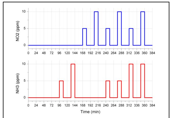
Figure 8. Gas profile applied to the \text{WO}_3 sensitive layer with the temperature-modulated profile
