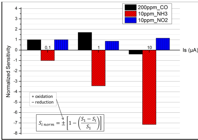
Figure 6. Normalized sensitivities of \text{WO}_3 sensitive layer to three different gases at 500^\circ\text{C}
