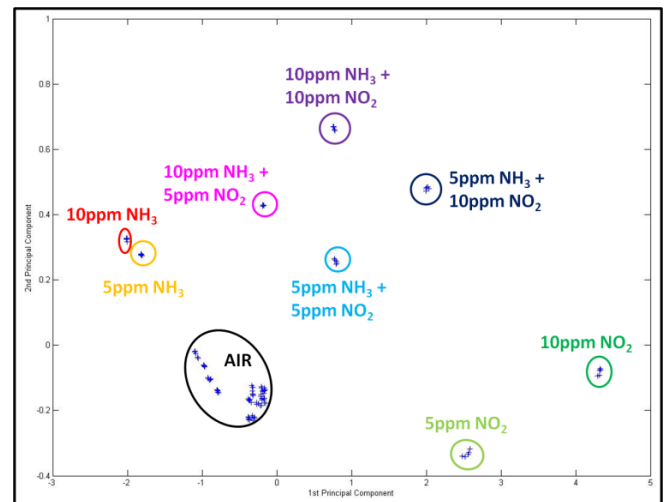
Figure 9. Principal component analysis of \text{WO}_3 sensitive layer
