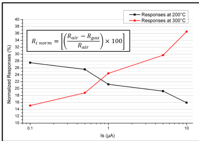
Figure 7. Normalized responses of \text{WO}_3 sensitive layer to \text{NH}_3 10 ppm for two different heater constant temperatures
