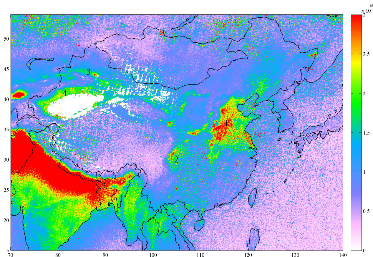
Fig. 13. \text{NH}_3 distribution over eastern Asia ( \text{molec cm}^{-2} ), following a gridding method explicitly accounting for the IASI footprint on each individual measurement. The distribution is a five-year error-weighted average of the IASI daytime total columns in the region (a post-filtering excluding cells with less than 10 observations has been carried out over land).
