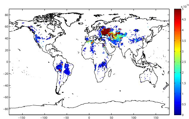
Fig. 2. IASI morning NH 3 observations (mole cm -2 ) on 15 August 2010 obtained using the FORLI processing chain. The high concentrations measured in eastern Europe are due to the exceptional emissions from the large Russian fires in the summer of 2010 (R'Honi et al., 2013).
