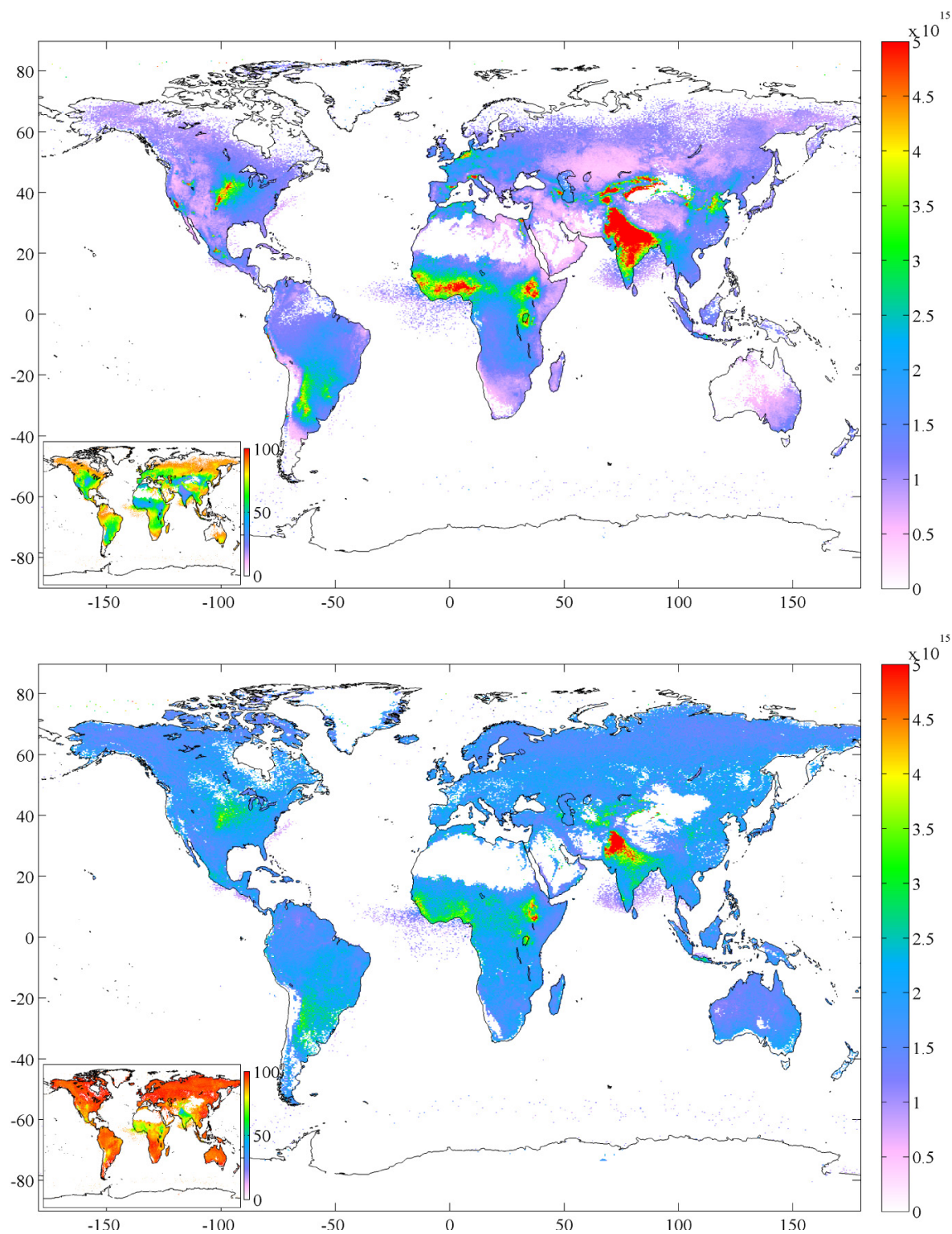
Fig. 11. NH 3 total columns (molec cm -2 ) and relative error (bottom-left inset, %) distributions for five years of IASI measurements (1 November 2007 to 31 October 2012), in 0.25^\circ \times 0.5^\circ cells for the morning (top panel) and evening (bottom panel) overpasses. The NH 3 distributions are a mean of all measurements within a cell, weighted by the absolute retrieval error following Eq. (3). The error distributions are a weighted mean of the absolute error of all observations within a cell following Eq. (4) and divided by the NH 3 total columns to provide an error distribution in %.
