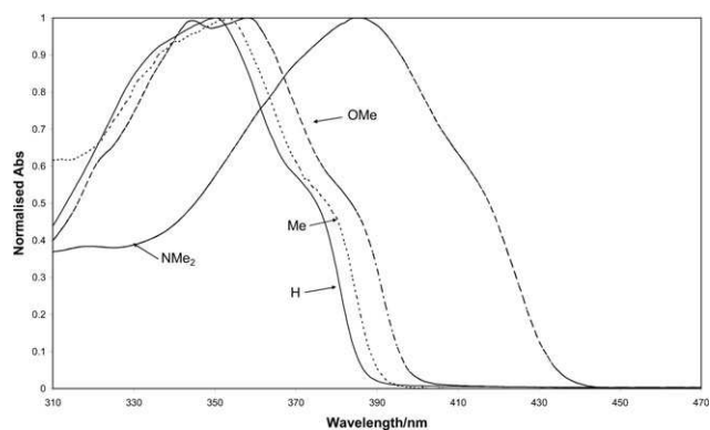
Fig. 1 Absorption spectra of compounds 1a–c and 1e .
