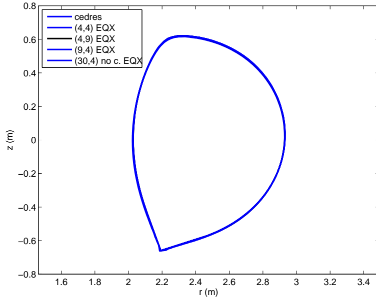
Figure 6. Plasma boundaries. Boundaries computed with Equinox (EQX) with (n^e = 4, n^i = 4) or (n^e = 9, n^i = 4) and (n^e = 30, n^i = 4) without any PF coils modelization (no c.) are almost superimposed with the reference boundary computed with Cedres. The boundary computed with Equinox (n^e = 4, n^i = 9) does not show any irregularities
