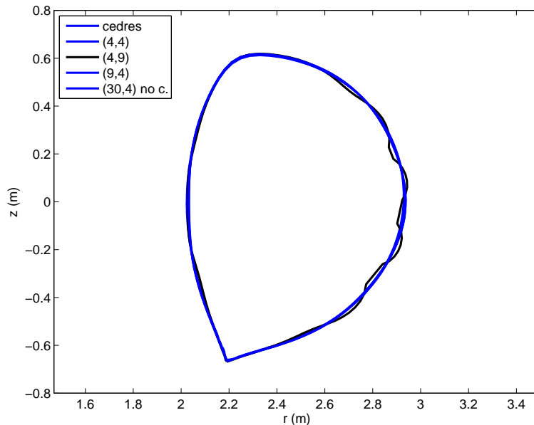
Figure 4. Plasma boundaries. Boundaries computed with ( n^e = 4, n^i = 4 ) or ( n^e = 9, n^i = 4 ) and ( n^e = 30, n^i = 4 ) without any PF coils modelization (no c.) are almost superimposed with the reference boundary computed with Cedres. The boundary computed with ( n^e = 4, n^i = 9 ) shows some irregularity
