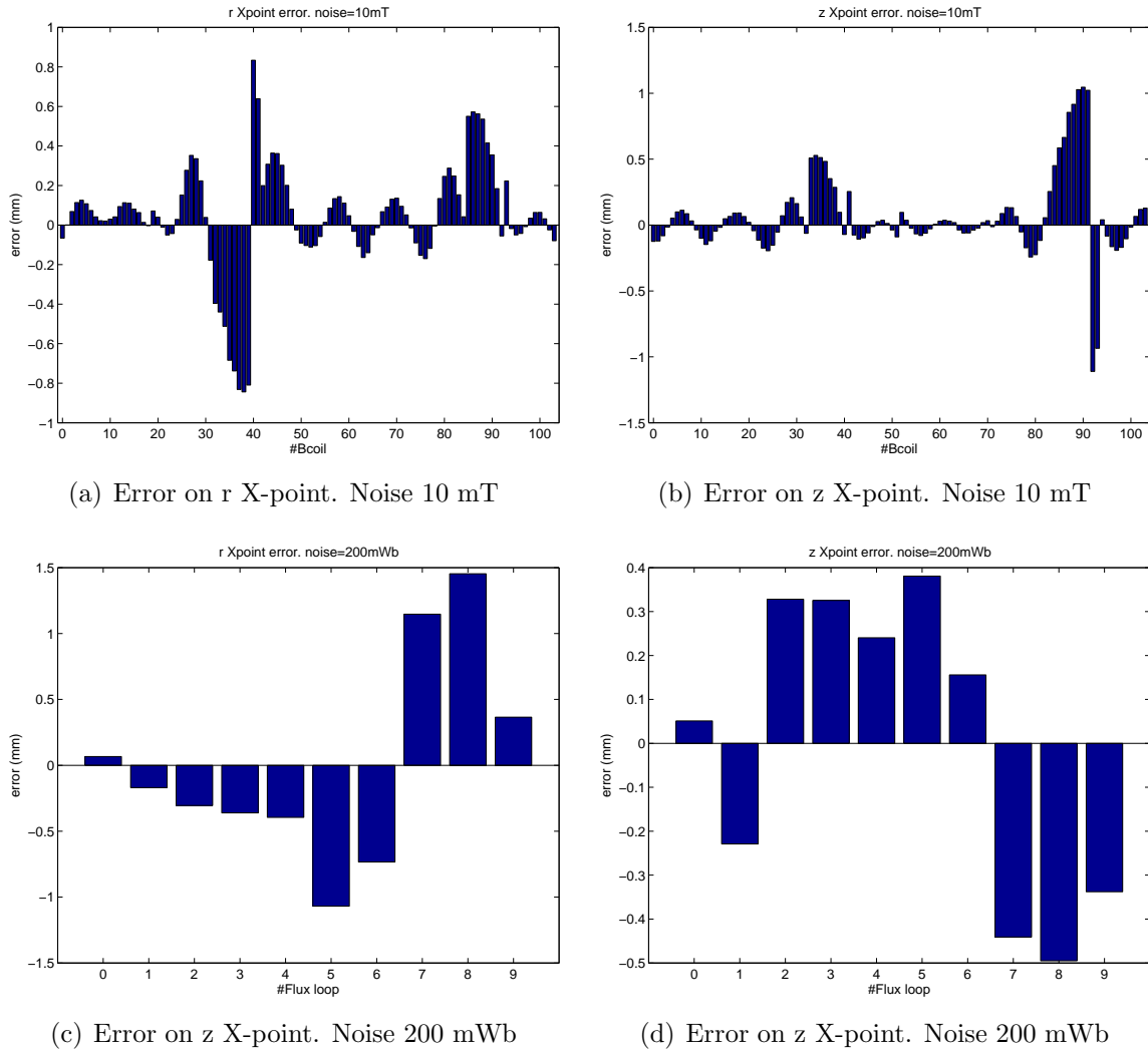
Figure 7. Error introduced on X-point position reconstruction by adding a 10 mT offset on a single Bcoil measurement or a 200 mWb offset on a single flux loop measurement.
