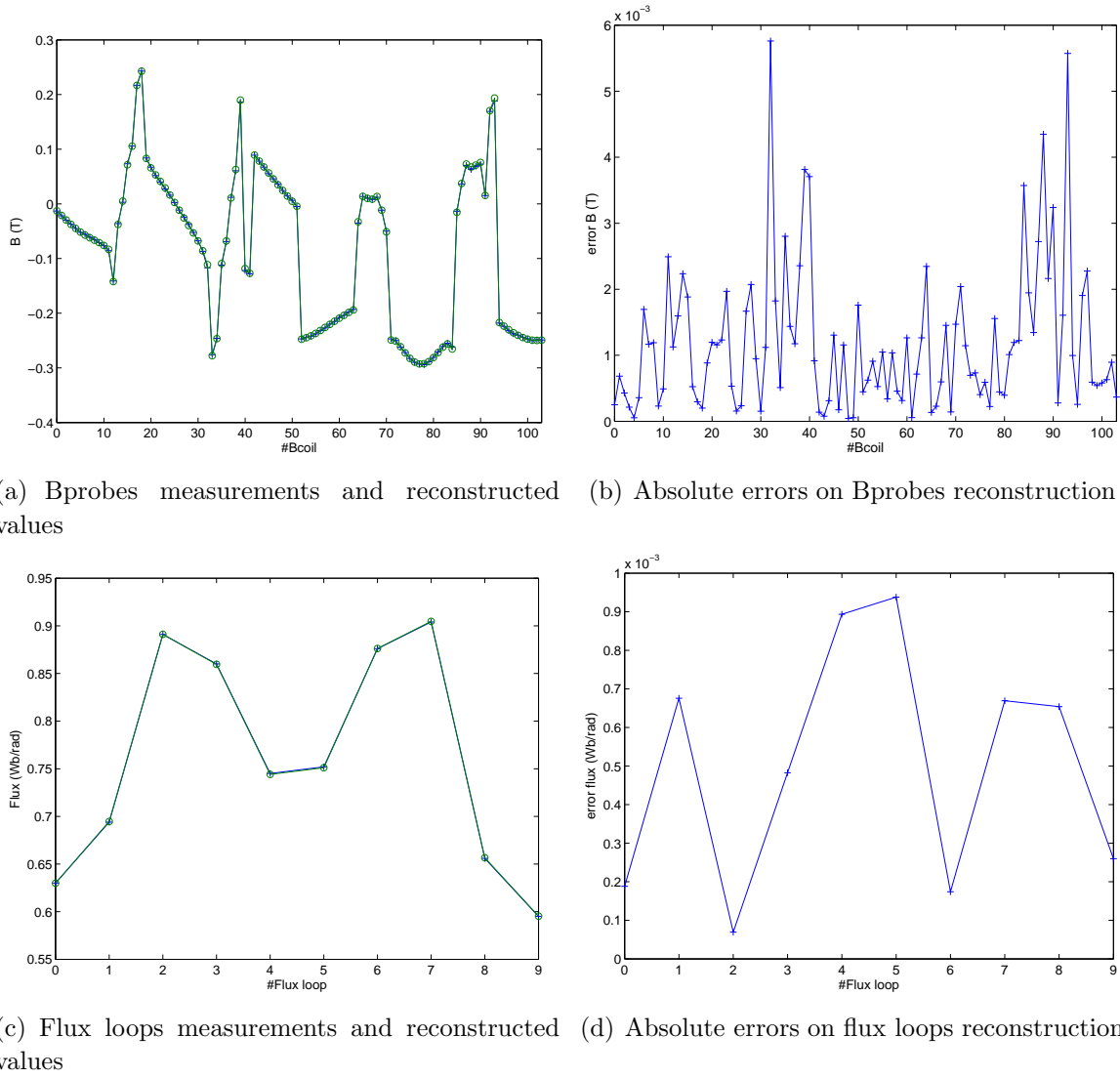
Figure 5. Comparison between measured and reconstructed values for WEST case 1 using (n^e = 4, n^i = 4) .
