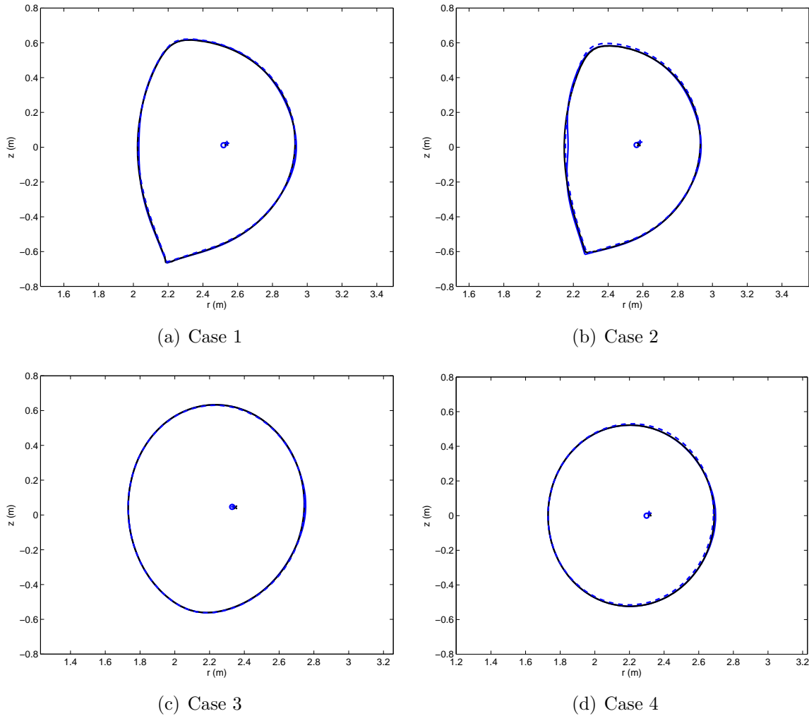
Figure 8. Cedres reference boundary (black), boundary reconstructed with toroidal harmonics (continuous blue line) and boundary reconstructed with Equinox (dashed blue line). Cedres and Equinox magnetic axis as well as the computed plasma center taken as the pole of the toroidal coordinate system (circle) are also shown.
