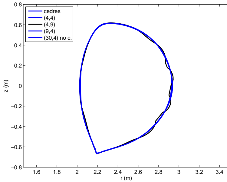
Figure 4. Plasma boundaries. Boundaries computed with ( n^e = 4, n^i = 4 ) or ( n^e = 9, n^i = 4 ) and ( n^e = 30, n^i = 4 ) without any PF coils modelization (no c.) are almost superimposed with the reference boundary computed with Cedres. The boundary computed with ( n^e = 4, n^i = 9 ) shows some irregularity
