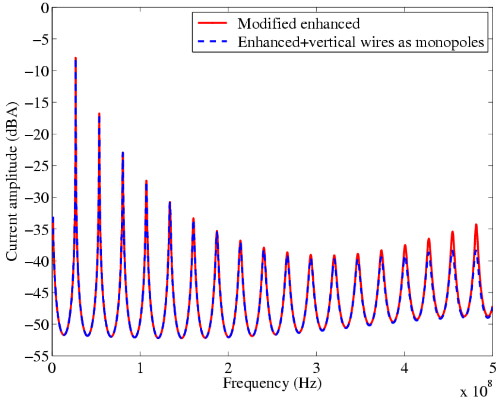
Figure 6. Current amplitude as a function of the frequency at the end of the TL, using the modified enhanced p.u.l. parameters and including the vertical wires.
