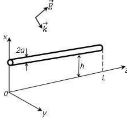
Figure 1. Geometry of the studied problem
