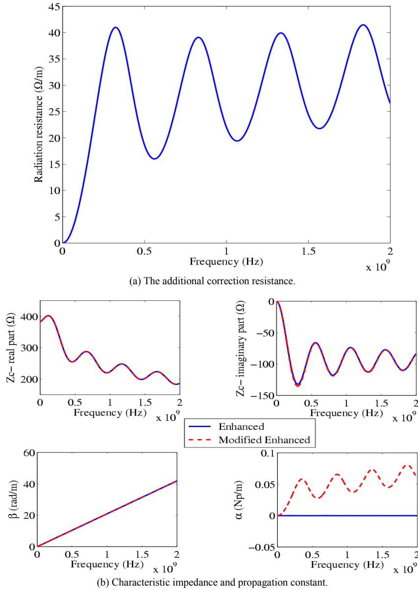
Figure 3. Characteristics of the modified enhanced p.u.l. parameters for a lossless TL above a PEC ground, height=0.3m, radius=1mm.
