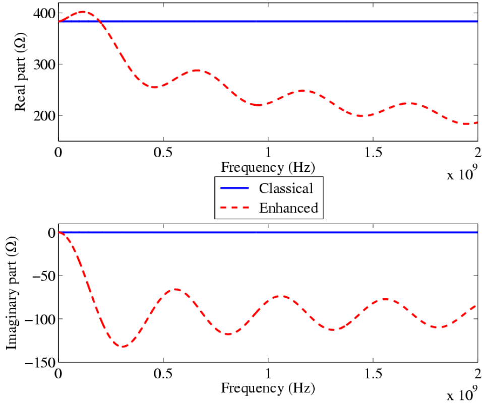
Figure 2. Comparison between the classical and enhanced characteristic impedance for a lossless TL above a PEC ground, height=0.3m, radius=1mm.
