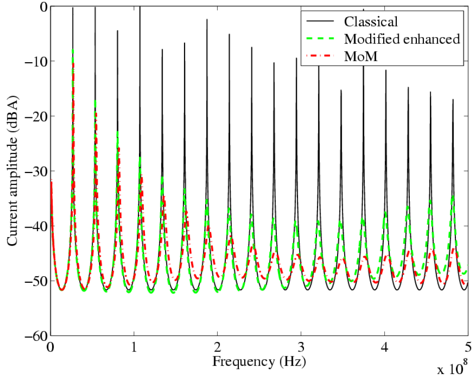
Figure 5. Current amplitude as a function of the frequency at the end of the TL, using the modified enhanced p.u.l. parameters.
