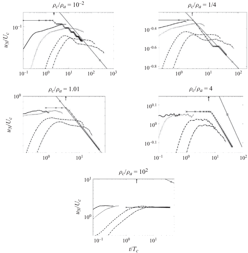
FIGURE 13. Temporal evolution of the front velocity at long times. Navier–Stokes simulations: —, \lambda = 18.75 ; \cdots , \lambda = 6.25 ; - - - -, \lambda = 1 ; - · - · - ·, \lambda = 0.5 . Shallow-water theory: — \times —, finite-difference solution of (2.1)–(2.4); — \square —, self-similar solution (2.7)–(2.9). For comparison, we indicate the value of t_S/T_c by an arrow.
