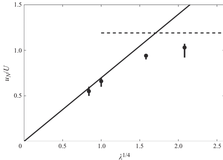
FIGURE 10. Front velocity as a function of \lambda^{1/4} for the light current ( \rho_c/\rho_a = 10^{-2} and H^* = 10 ). The symbols correspond to time average and the error bar indicates the range of values taken by the front velocity over this range (see figure 5 caption for details). Lines: —, prediction of (4.4); - - - - -, predicted slumping front velocity from the shallow-water theory (2.3)–(2.5).
