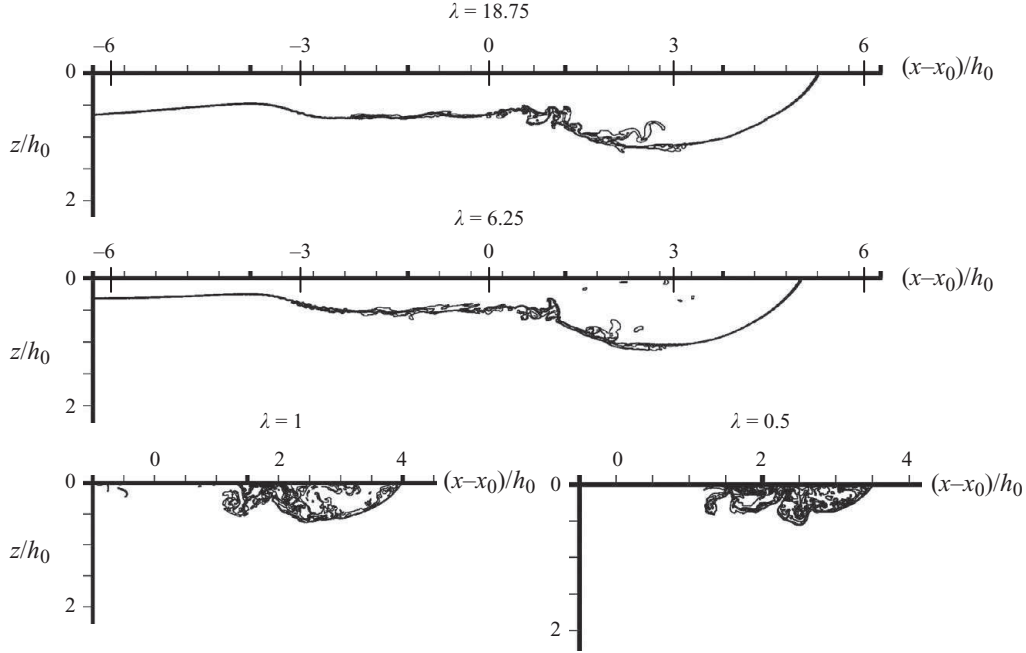
FIGURE 8. Same as figure 7 for light top density currents ( \rho_c/\rho_a = 10^{-2} ) at the time instant t/T \approx 5.6 .
