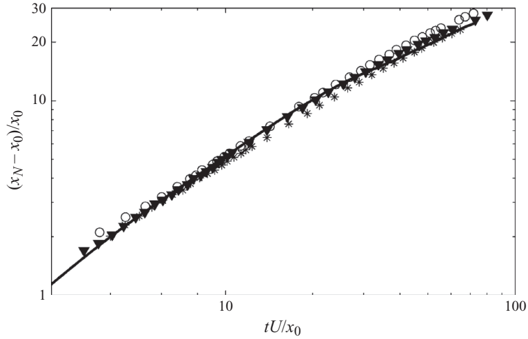
FIGURE 2. Evolution of the front position in Boussinesq currents for partial depth releases ( H^* > 1 ). Experiments of Marino et al. (2005): (*) run 13: H^* \approx 1.5 , \lambda \approx 0.37 , Re \approx 4 \times 10^4 ; (O) run 18: H^* \approx 1.6 , \lambda \approx 0.41 , Re \approx 6 \times 10^4 ; (▼) run 19: H^* \approx 1.9 , \lambda \approx 0.47 , Re \approx 2.7 \times 10^4 . Present Navier–Stokes simulation: —, same parameters as in run 19.
