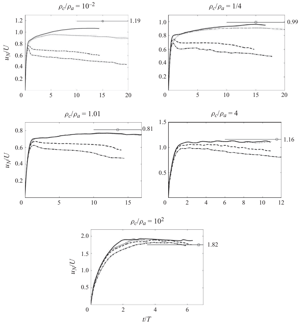
FIGURE 3. Temporal evolution of the front velocity u_N for various lock aspect ratios \lambda and density ratios \rho_c/\rho_a : —, \lambda = 18.75 ; \cdots , \lambda = 6.25 ; - - - - -, \lambda = 1 ; - · - · - ·, \lambda = 0.5 . The horizontal lines with circle represent the slumping velocity u_{SW} predicted by the shallow-water theory (2.3)–(2.5). Here u_N and t are scaled by U and T , respectively, as defined in (1.1).
