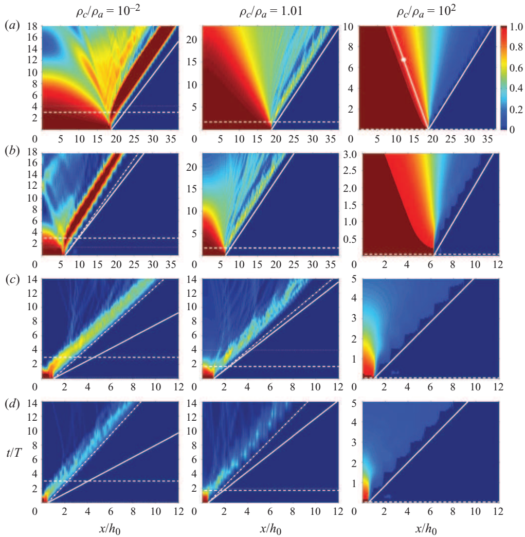
FIGURE 9. (Colour online at http://journals.cambridge.org/flm ) Space–time diagram showing the height \bar{h}(x,t) , as defined by (4.1), of the Boussinesq and non-Boussinesq density currents: (a) \lambda = 18.75 ; (b) \lambda = 6.25 ; (c) \lambda = 1 ; (d) \lambda = 0.5 . Lines: —, shallow-water solution (2.3)–(2.5) in the slumping regime; -·-·-, solution (4.4); ·····, t_S as defined in (4.10); - - - - -, t_H as defined in (4.13). Note that the observed ‘steps’ at the front of the current are due to the limited number of time samples used for the generation of the diagrams, and are in no way a solution of the Navier–Stokes equations (as is evident from the temporal evolution of u_N in figure 3). The line with circle in the case of the largest \rho_c/\rho_a and \lambda is x/t = -U , i.e. the speed of the rarefaction wave as predicted by the shallow-water theory for the dam-break problem.
