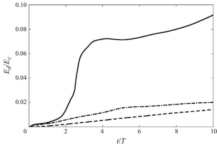
FIGURE 4. Temporal evolution of the ratio of dissipation E_d to kinetic energy E_c ( H^* = 10 , Re = 25\,000 ): —, \rho_c/\rho_a = 10^{-2} ; - - - - -, \rho_c/\rho_a = 1.01 ; - · - · - ·, \rho_c/\rho_a = 10^2 . Observe that for Boussinesq and bottom currents, the dissipation is only a few per cent of the kinetic energy.
