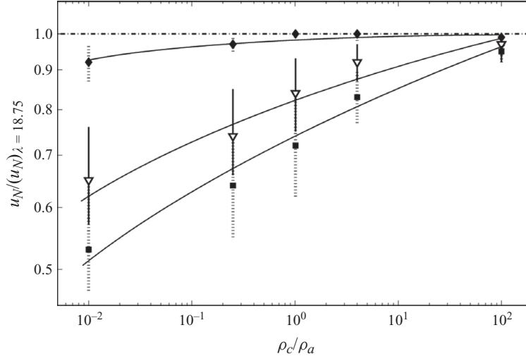
FIGURE 5. Influence of the lock aspect ratio measured in terms of ratio of front velocity at small \lambda to the front velocity for the \lambda = 18.75 case, plotted as a function of density ratio for varying values of \lambda . The symbols correspond to the ratio of time-averaged front velocity, where the average is taken over the time interval [T_I, T_F] . Here, T_I is chosen so that the initial acceleration phase is excluded ( T_I/T > 2 ) and T_F is chosen so that the current spreads over a distance of 10h_0 ( 6 < T_F/T < 15 depending on the density ratio). In several cases, the front velocity continually changes over time and as a consequence we also plot a vertical bar that indicates the range of values the ratio will take if it were computed based on instantaneous u_N/(u_N)_{\lambda=18.75} taken over this interval. Symbols: \blacklozenge , \lambda = 6.25 ; \nabla , \lambda = 1 ; \blacksquare , \lambda = 0.5 . Lines are plotted to show tendency.
