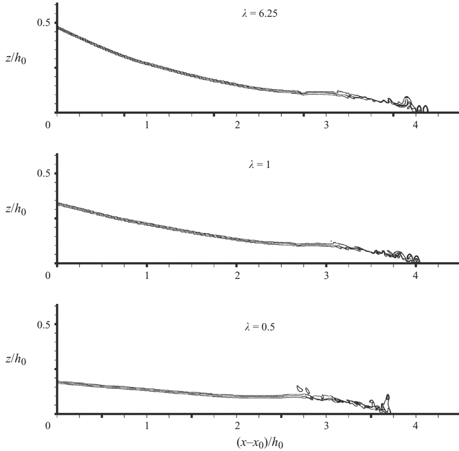
FIGURE 6. Instantaneous shape of heavy currents ( \rho_c/\rho_a = 10^2 ) at the time instant t/T = 2.8 . Isolines of (\rho - \rho_a)/(\rho_c - \rho_a) = 0.1, 0.5 and 0.9 are shown. Observe that the pictures have been stretched out in the vertical direction by a factor of 2, owing to the elongated shape of the currents.
