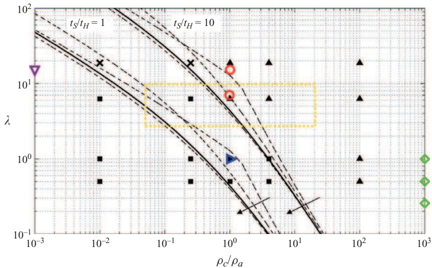
FIGURE 12. (Colour online) Contours t_S/t_H = 1 and t_S/t_H = 10 in the parameter space ( \rho_c/\rho_a ; \lambda ), t_S and t_H being calculated via (4.9) and (4.13), respectively. The thick solid lines are for H^* = 10 , while the thin dashed lines are for H^* = 1, 2 and 10^3 (following the arrow). The locations in the parameter space of the Navier–Stokes simulations are represented by the symbols corresponding to various \lambda -dependences of the front speed: \blacktriangle , no dependence; \blacksquare , significant dependence; \times , possible dependence. Also plotted are the locations of large H^* experimental results (see table 3 for legend).
