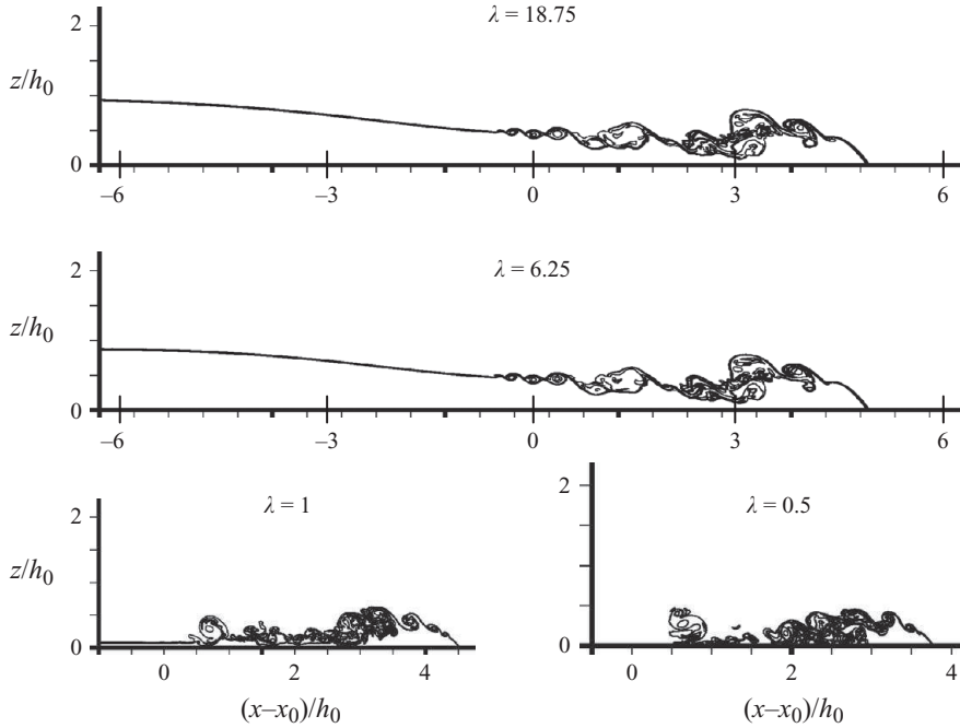
FIGURE 7. Instantaneous shape of Boussinesq density currents ( \rho_c/\rho_a = 1.01 ) at the time instant t/T \approx 7 . Isolines of (\rho - \rho_a)/(\rho_c - \rho_a) = 0.05, 0.25, 0.5, 0.75 and 0.95 are shown.
