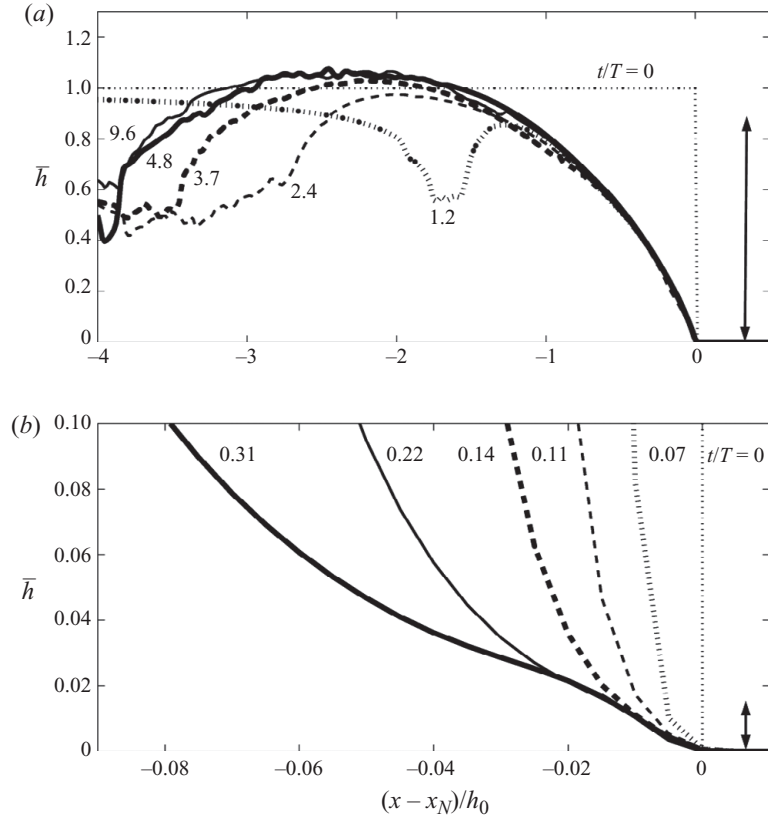
FIGURE 11. Temporal evolution of the equivalent height \bar{h} at the front of the current, obtained from the Navier–Stokes simulations, for (a) a light current ( \rho_c/\rho_a = 10^{-2} ; \lambda = 6.25 ) and (b) a heavy current ( \rho_c/\rho_a = 10^2 ; \lambda = 6.25 ). For comparison, the height of the current h_N as predicted by the shallow-water theory (2.6) is indicated by an arrow. Observe that the time of formation of the heavy current head is much smaller than that of the light current.
