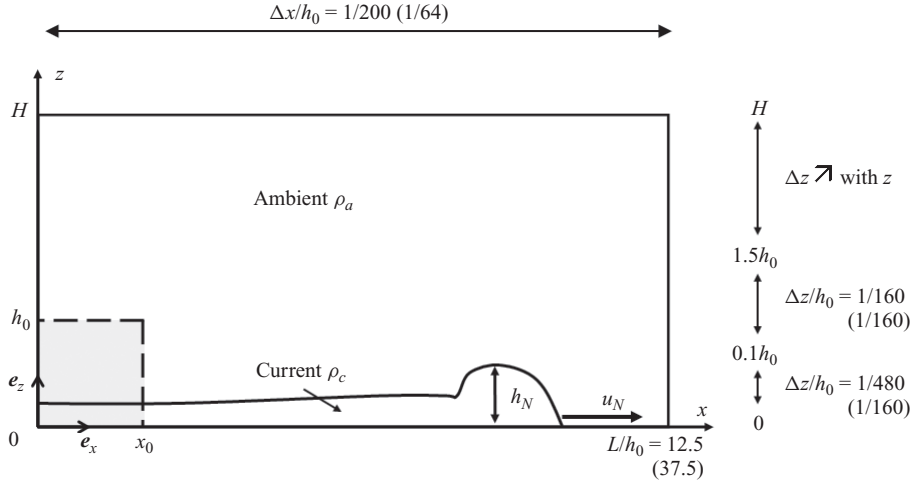
FIGURE 1. Physical configuration used in the present work and spatial resolution of the Navier–Stokes simulations. The dashed line represents the initial separation between the current and the ambient, while the solid line represents the interface at later times. The gravitational acceleration \mathbf{g} acts in the negative z -direction of unit vector \mathbf{e}_z . The bottom and top of the channel are at z=0 and z=H , respectively. Light currents propagate along the top boundary and the vertical resolution is inverted accordingly. Here, u_N is the instantaneous speed of the current and h_N is defined as the maximum height of the nose of the current. The spatial resolution is identical for all \lambda except \lambda=18.75 for which the resolution is given in parentheses.
