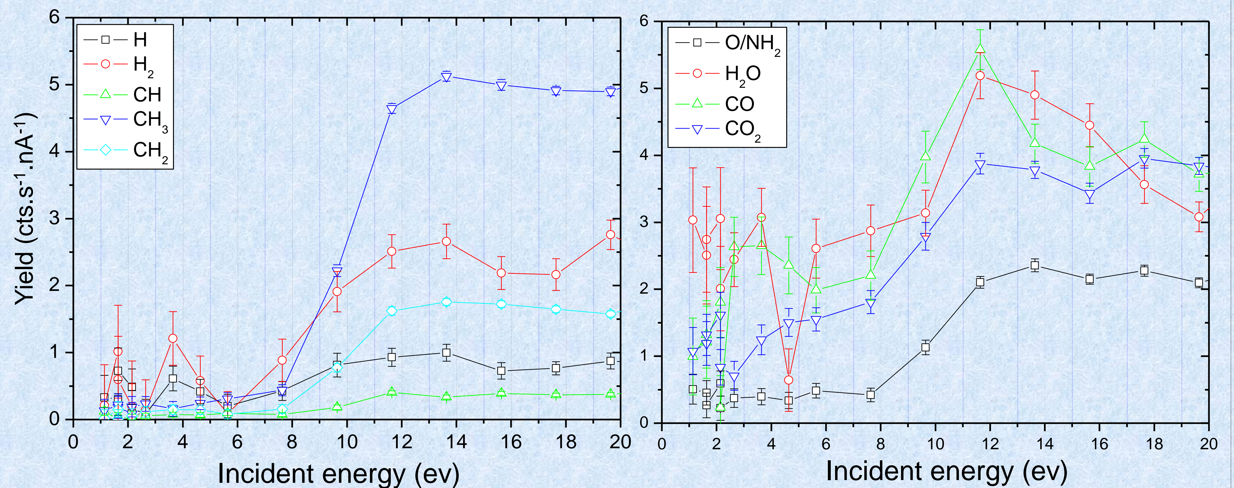
Fig. (6) Yields of neutral species desorbing from a DNA-Dap thin film (10 nm thickness) versus the irradiation electron energy. Some species exhibit resonant structures at very low energy (around 1.5 and 3.5 eV). We attribute these resonant features to the TNIs observed by electrophoresis at 0.8, 0.3 and 2.2 eV [6]. Above 6 eV, most of the desorption yields increase with a broad resonant structure around 13 eV.
