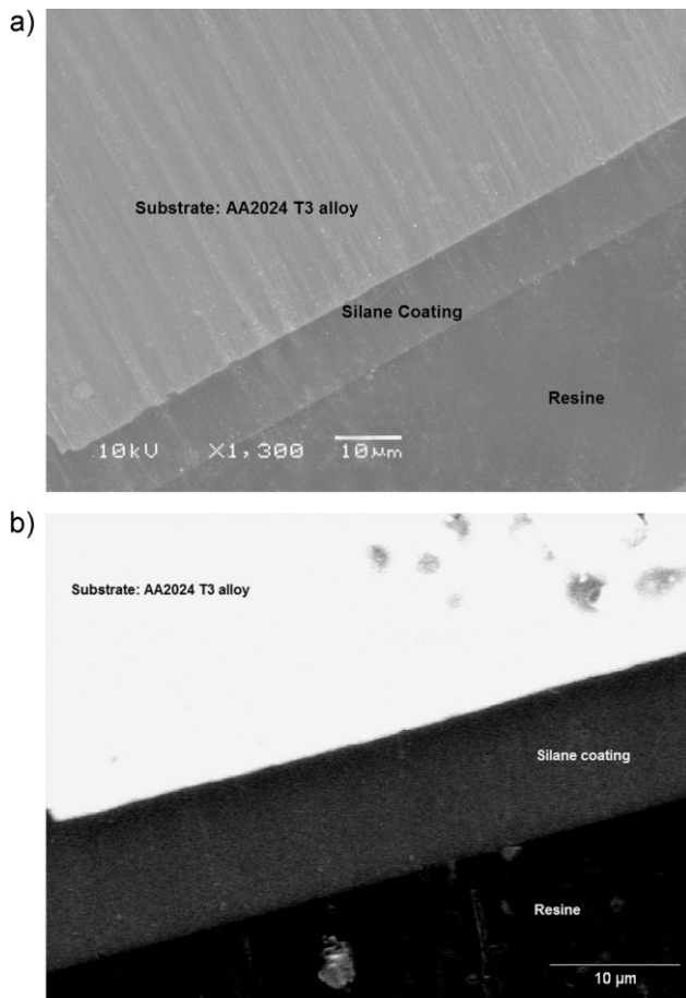
Figure 1. SEM for AA2024-T3 [0.01]Ce sample: a) secondary electrons, b) backscattered electrons
