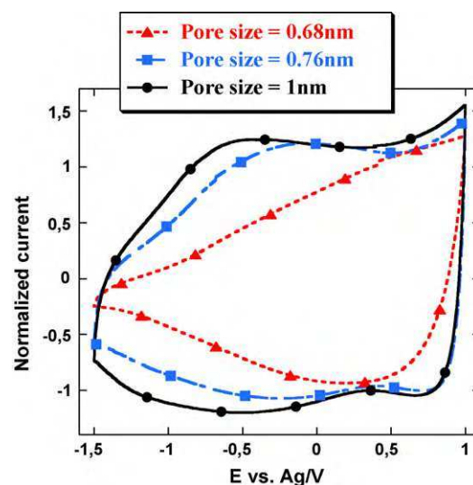
Fig. 2. Normalized CVs of the three CDC samples in PC + 1 M \text{NEt}_4\text{BF}_4 electrolyte between -1.5\ \text{V}/\text{Ref} and 1.0\ \text{V}/\text{Ref} . Scan rate: 100 mV/s.
