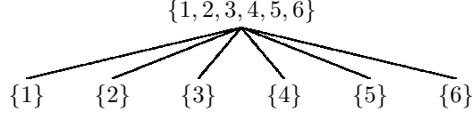
Figure 2.1: A dimension partition tree related to \mathbf{V}_D = {}_a \bigotimes_{j=1}^6 V_j .
